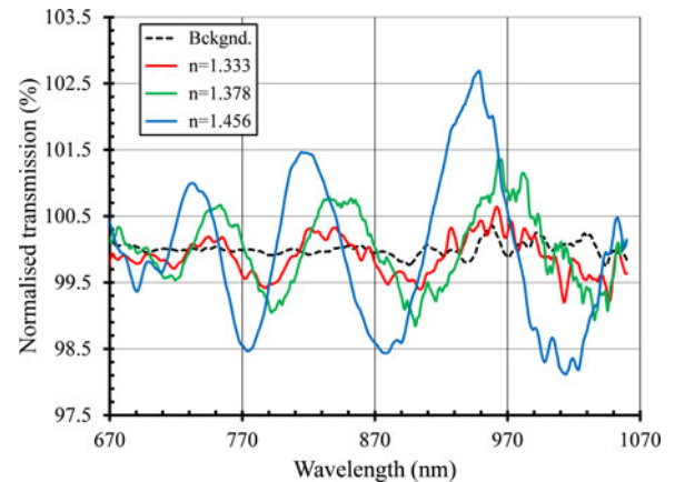
Fig. 8. Transmission change of a 6 taper TPLG with a waist diameter of 117 \mu\text{m} when it is immersed in liquids with an index ranging from 1.333–1.456. The fiber used was SM750.
