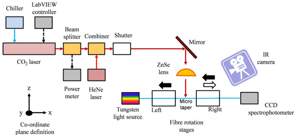
Fig. 1. Schematic of the TLPG fabrication system. When the micro-taper is formed the stages rotate in opposite directions. During fiber translation the stages rotate in the same direction.
