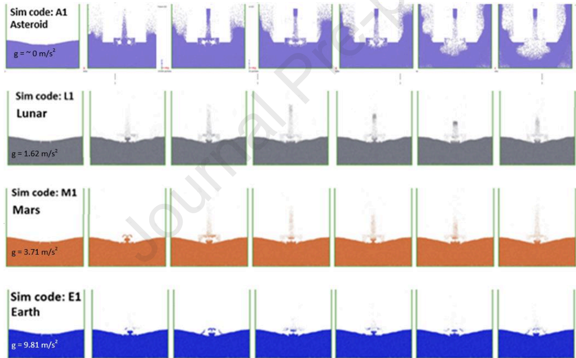
Figure 5-5 Particle flow comparison at various space bodies with 100rpm rotation speed. Sampling time from left to right, t = 0s, 0.25s, 0.5s, 0.75s, 1s, 1.5s , and 2s . Images are sliced and viewed from the x-z-axis.
