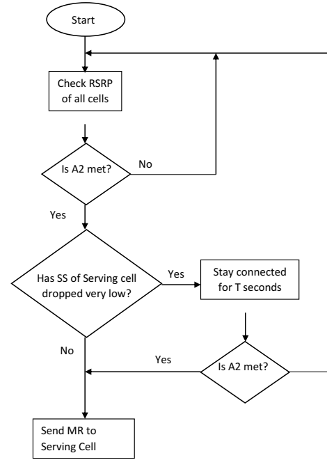
Fig.2. Algorithm 1 flowchart.
