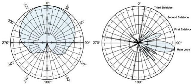
Fig. 5. Katherin 800 10123 antenna radiation pattern at 1710-2180 Mhz.
