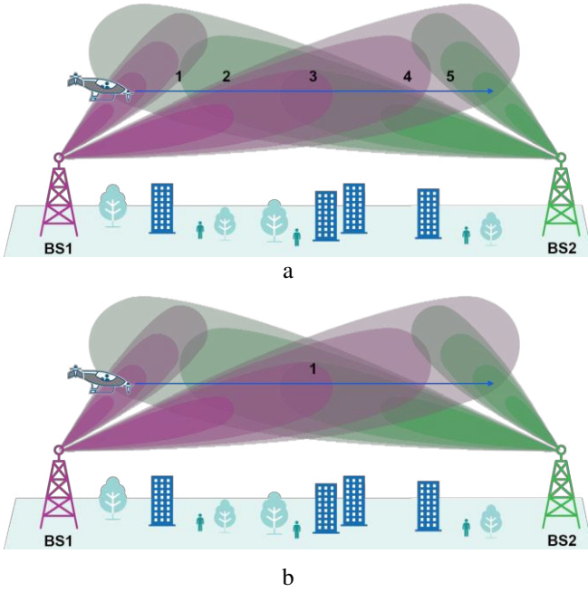
Fig. 1. a) unnecessary ping-pong handovers due to sidelobes null spaces. b) minimized handovers through modified LTE handover procedure.
