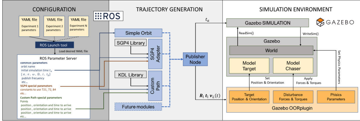
Fig. 1. OnOrbitROS architecture
