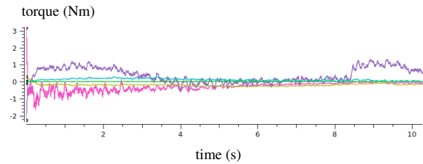
Fig. 7. Control action (torque) during the tracking
