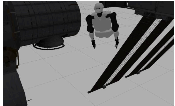
Fig 3. OnOrbitROS simulation of the humanoid robot
