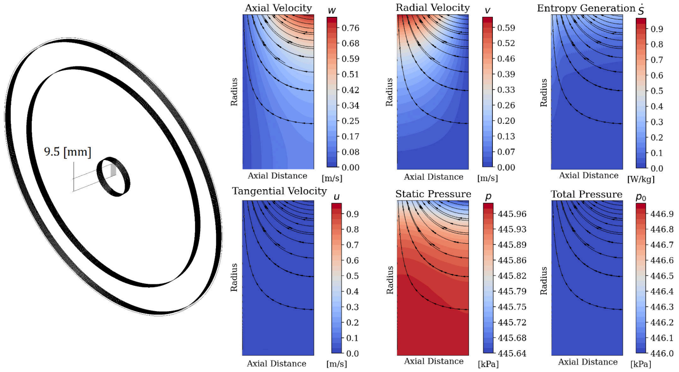
FIGURE 5: CROSS-SECTIONAL CONTOUR OF ROTOR-ONLY MODEL ALONG THE 0 DEGREE RADIAL IN THE RADIUS RANGE OF 0 [MM] < R < 9.5 [MM] (INLET REGION). PRESENTED PARAMETERS ARE AXIAL, RADIAL, TANGENTIAL VELOCITIES, TOTAL AND STATIC PRESSURE, AND ENTROPY GENERATION RATE.
