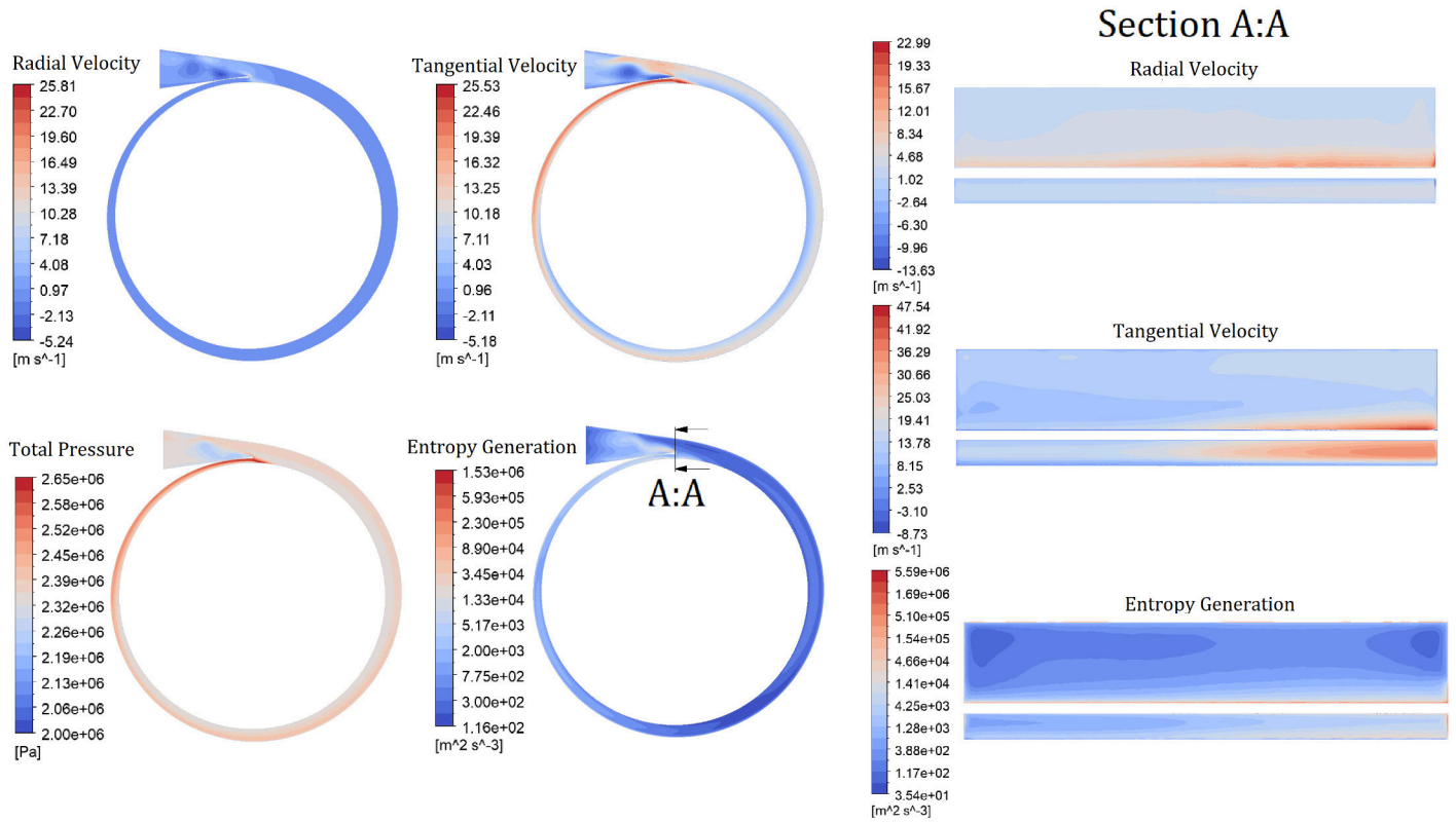
FIGURE 12: FLOW FIELD RESULTS FROM VOLUTE-ONLY MODEL. PRESENTED PARAMETERS ARE RADIAL AND TANGENTIAL VELOCITY, TOTAL PRESSURE, AND ENTROPY GENERATION. A CROSS-SECTIONAL VIEW AT THE VOLUTE TONGUE IS ALSO PRESENTED.
