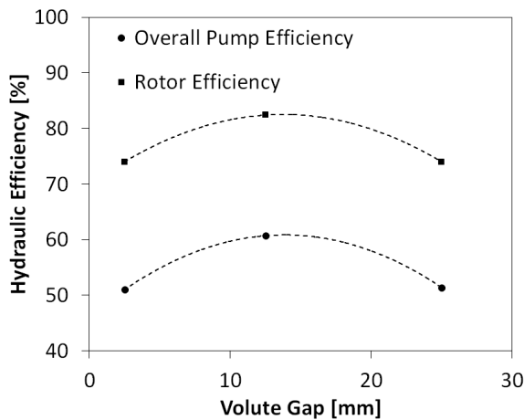
FIGURE 25: CFD RESULTS OF HYDRAULIC EFFICIENCY OF BOUNDARY LAYER PUMP MODELS AGAINST VOLUTE TONGUE GAP CLEARANCE.
