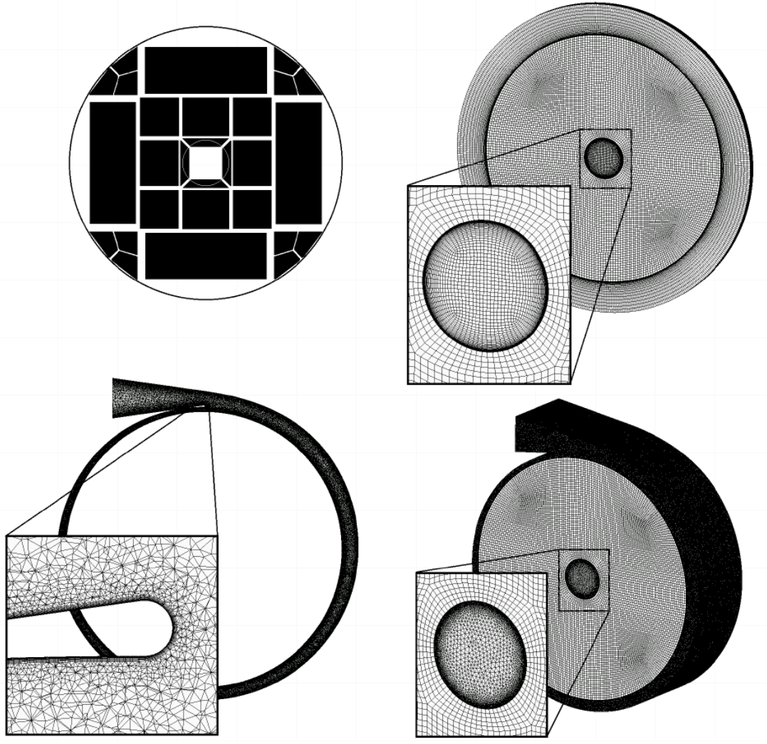
FIGURE 4: DEVELOPED GRIDS FOR THE THREE MODELS. (TOP LEFT) – GRID TOPOLOGY FOR DISC GAPPED SPACE. (TOP RIGHT) – BASELINE MODEL WITH ONE-TENTH THE NUMBER OF DISCS AND ARTIFICIAL OUTLET DOMAIN. (BOTTOM LEFT) – VOLUTE OUTLET CHANNEL GRID. (BOTTOM RIGHT) – INTEGRATED MODEL WITH 170 DISCS AND VOLUTE CHANNEL.
