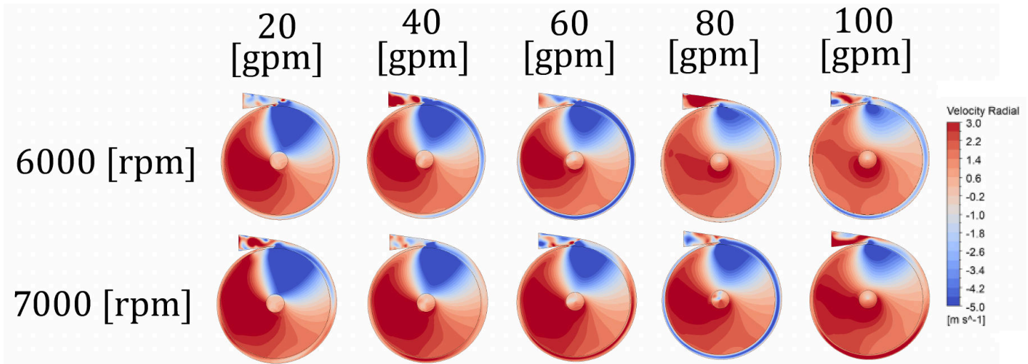
FIGURE 16: RADIAL VELOCITY CONTOURS AT HALF-THICKNESS OF THE INTEGRATED MODEL FOR 5 DIFFERENT MASS FLOW RATES AND 2 ROTATIONAL SPEEDS.
