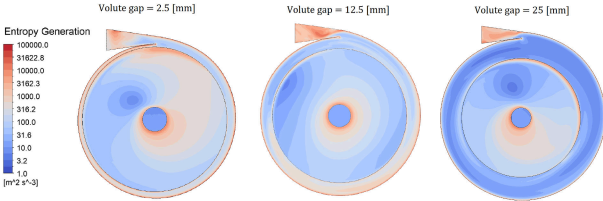
FIGURE 22: SECTION VIEW OF ENTROPY GENERATION RATE AT HALF-THICKNESS OF THREE BOUNDARY LAYER PUMPS WITH DIFFERENT VOLUTE TONGUE GAP CLEARANCES
