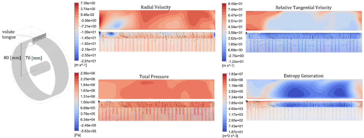
FIGURE 15: CROSS-SECTIONAL CONTOUR OF INTEGRATED MODEL ALONG THE 0 DEGREE RADIAL IN THE RADIUS RANGE OF 70 [MM] < R < 87 [MM] (ROTOR-VOLUTE INTERFACE UNDERNEATH VOLUTE TONGUE). PRESENTED PARAMETERS ARE RADIAL AND RELATIVE TANGENTIAL VELOCITIES, TOTAL PRESSURE, AND ENTROPY GENERATION RATE.
