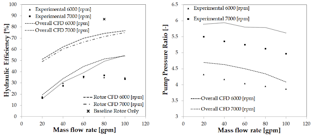
FIGURE 19: HYDRAULIC EFFICIENCY (LEFT) FOR OVERALL PUMP EXPERIMENTAL AND CFD RESULTS AND FOR CFD RESULTS FROM INTEGRATED MODEL ACROSS THE ROTOR. PRESSURE RATIO (RIGHT) FOR EXPERIMENTAL AND CFD RESULTS FOR THE OVERALL PUMP.
