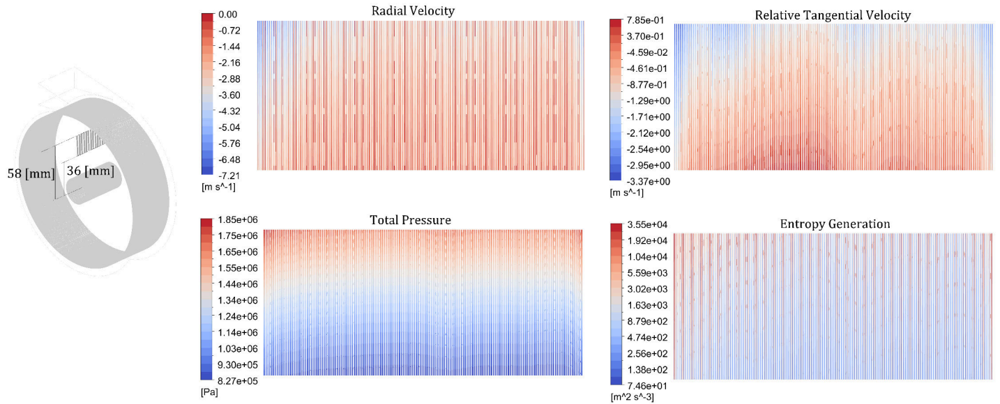
FIGURE 14: CROSS-SECTIONAL CONTOUR OF INTEGRATED MODEL ALONG THE 0 DEGREE RADIAL IN THE RADIUS RANGE OF 36 [MM] < R < 58 [MM]. PRESENTED PARAMETERS ARE RADIAL AND RELATIVE TANGENTIAL VELOCITIES, TOTAL PRESSURE, AND ENTROPY GENERATION RATE.
