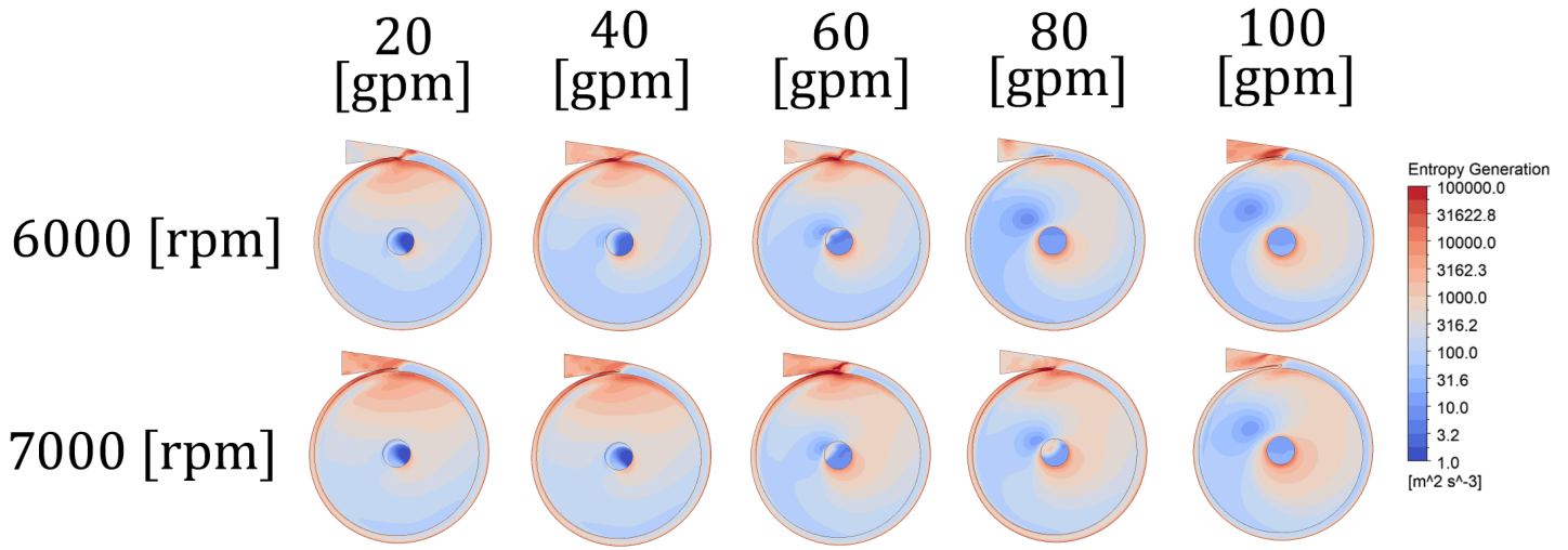
FIGURE 18: ENTROPY GENERATION CONTOURS AT HALF-THICKNESS OF THE INTEGRATED MODEL FOR 5 DIFFERENT MASS FLOW RATES AND 2 ROTATIONAL SPEEDS.
