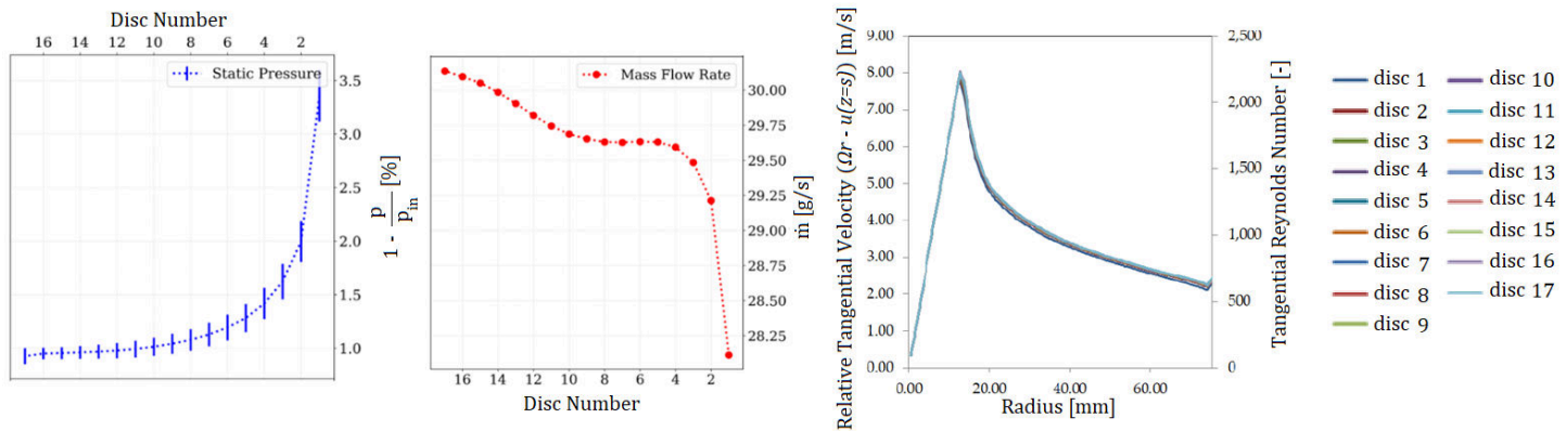
FIGURE 7: FLOW PROPERTIES AT THE INTER-DISC GAPS INTERFACING WITH THE INLET REGION. (LEFT) – STATIC PRESSURE DROP ACROSS THE INTER-DISC GAPS. (MIDDLE) – MASS FLOW RATE VARIATION ACROSS DIFFERENT INTER-DISC GAPS. (RIGHT) – RELATIVE TANGENTIAL VELOCITY AND TANGENTIAL REYNOLDS NUMBER ACROSS THE ROTOR RADIUS.
