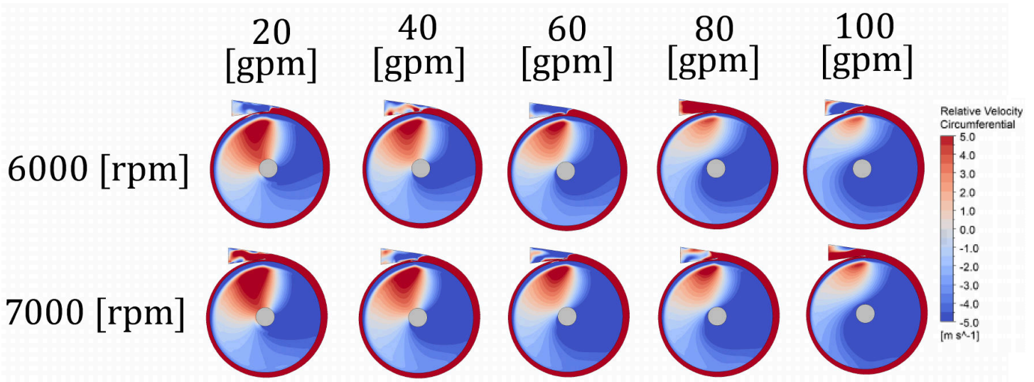
FIGURE 17: TANGENTIAL VELOCITY CONTOURS AT HALF-THICKNESS OF THE INTEGRATED MODEL FOR 5 DIFFERENT MASS FLOW RATES AND 2 ROTATIONAL SPEEDS.
