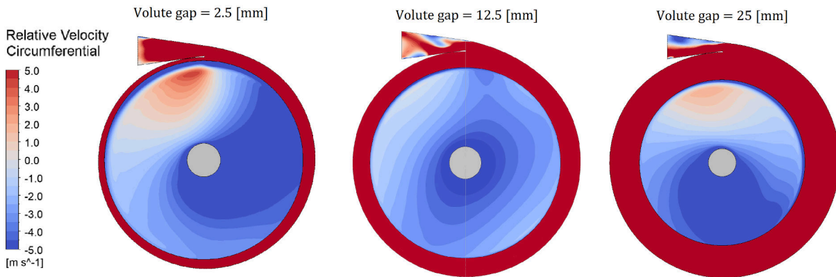
FIGURE 21: SECTION VIEW OF RELATIVE TANGENTIAL VELOCITY AT HALF-THICKNESS OF THREE BOUNDARY LAYER PUMPS WITH DIFFERENT VOLUTE TONGUE GAP CLEARANCES
