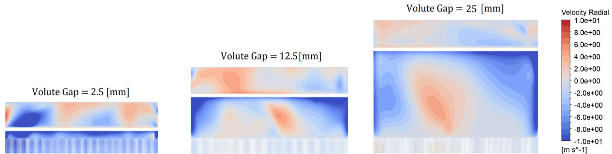
FIGURE 24: SECTION VIEW OF RADIAL VELOCITY ALONG THE ZERO-DEGREE RADIAL AT THE INTERFACE BETWEEN THE ROTOR AND VOLUTE FOR THREE BOUNDARY LAYER PUMPS WITH DIFFERENT VOLUTE TONGUE GAP CLEARANCES
