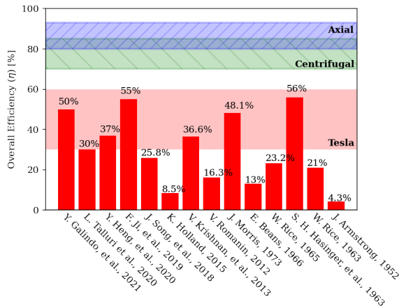
FIGURE 1: A COLLECTION OF BOUNDARY LAYER / TESLA TURBOMACHINERY (PUMPS AND TURBINES) EFFICIENCIES OBTAINED EXPERIMENTALLY.[1–6, 10–17]. FOR COMPARISON, TYPICAL CENTRIFUGAL [20] AND AXIAL [21] TURBOMACHINERY EFFICIENCIES ARE ALSO PLOTTED.
