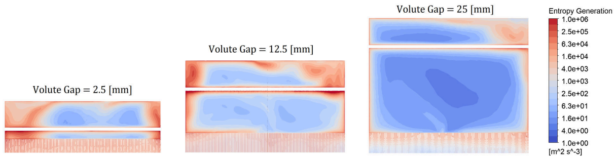
FIGURE 23: SECTION VIEW OF ENTROPY GENERATION RATE ALONG THE ZERO-DEGREE RADIAL AT THE INTERFACE BETWEEN THE ROTOR AND VOLUTE FOR THREE BOUNDARY LAYER PUMPS WITH DIFFERENT VOLUTE TONGUE GAP CLEARANCES
