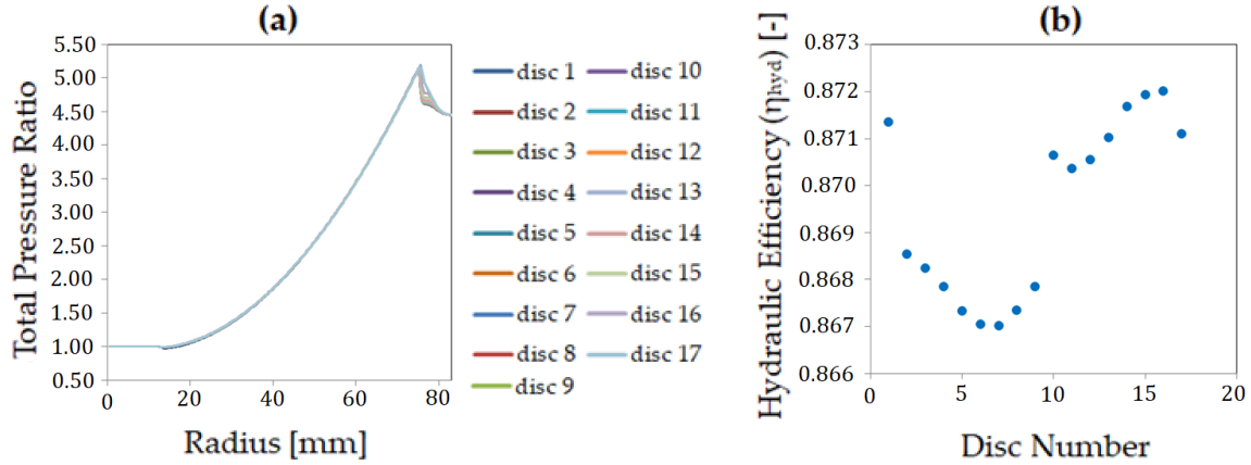
FIGURE 10: ROTOR TOTAL PRESSURE RATIO (A) AGAINST PUMP RADIUS FOR EACH INTER-DISC GAP OF THE ROTOR-ONLY MODEL. ROTOR HYDRAULIC EFFICIENCY OF ROTOR-ONLY MODEL (B) FOR EACH INTER-DISC GAP.
