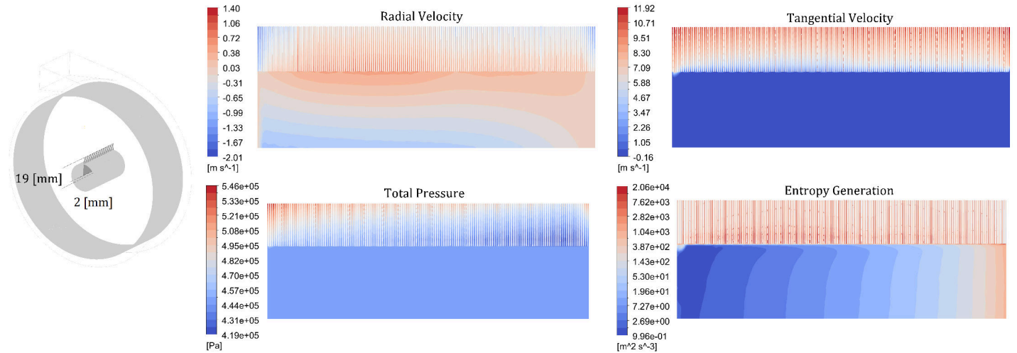
FIGURE 13: CROSS-SECTIONAL CONTOUR OF INTEGRATED MODEL ALONG THE 0 DEGREE RADIAL IN THE RADIUS RANGE OF 2 [MM] < R < 19 [MM]. PRESENTED PARAMETERS ARE RADIAL AND TANGENTIAL VELOCITIES, TOTAL PRESSURE, AND ENTROPY GENERATION RATE.
