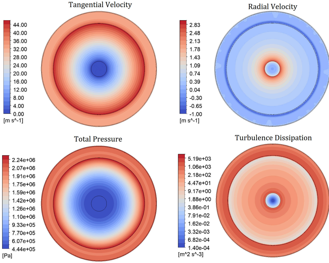
FIGURE 11: CROSS-SECTIONAL VIEW AT HALF-THICKNESS OF THE ROTOR IN THE ROTOR-ONLY MODEL.
