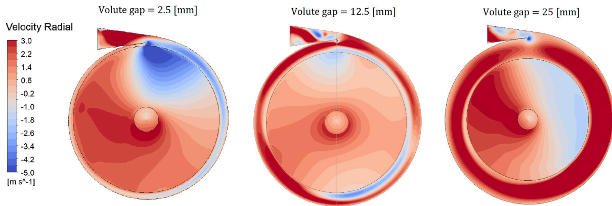
FIGURE 20: SECTION VIEW OF RADIAL VELOCITY AT HALF-THICKNESS OF THREE BOUNDARY LAYER PUMPS WITH DIFFERENT VOLUTE TONGUE GAP CLEARANCES
