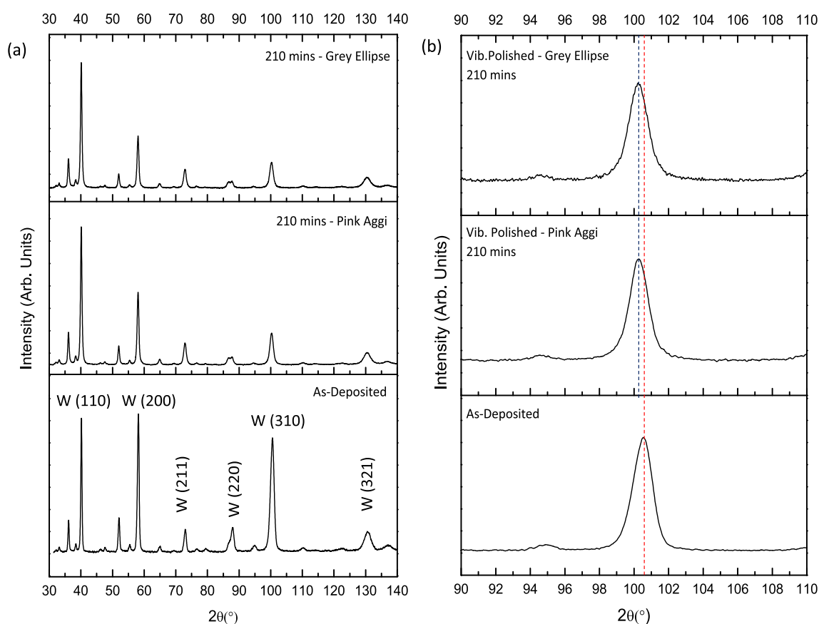
Fig. 10. XRD diffractogram of (a) as-deposited and vibratory polished W/WC coatings using Pink Aggi and Grey Ellipse media for a duration of 210 min and (b) a shift of the W {310} peak.
