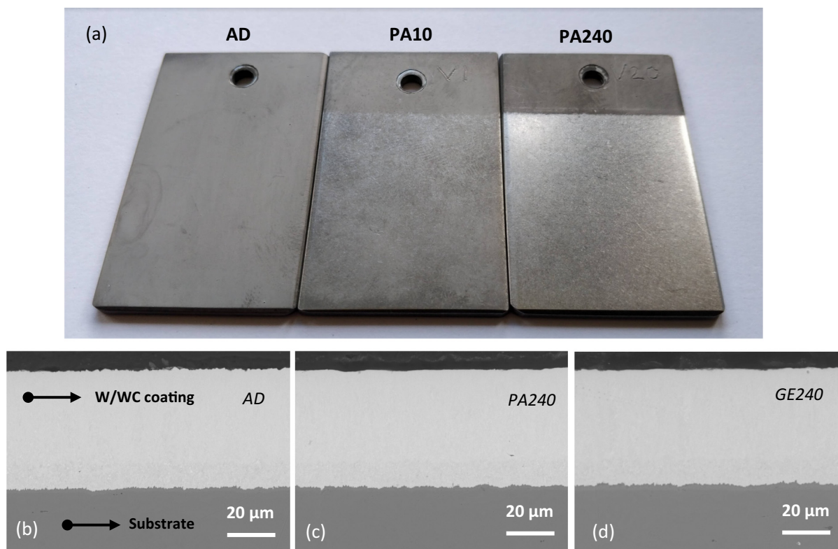
Fig. 1. (a) Photograph of W/WC coated samples in the AD, PA10 and PA240 conditions, cross-sectional SEM images of (b) AD prior to (c) PA240 testing and (d) GE240 testing.
