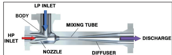
Fig. 4. Key components of a surface jet pump (SJP)
