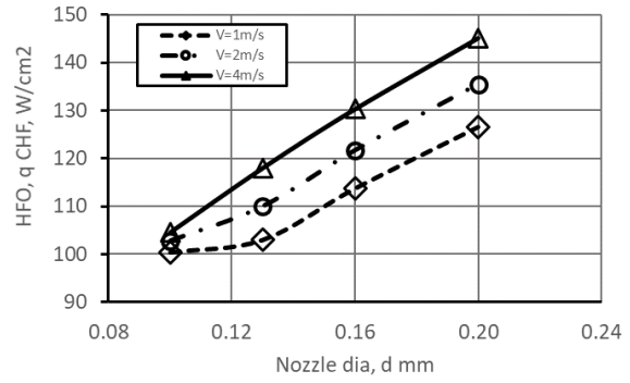
Figure 9: CHF at varying velocity for HFO
