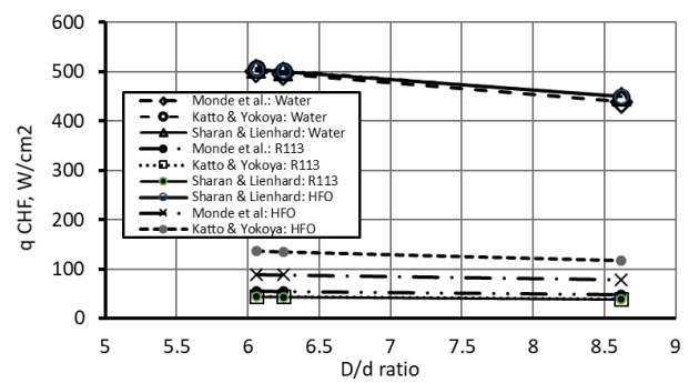
Figure 7: Critical heat flux with d/D ratio relation with different CHF models
