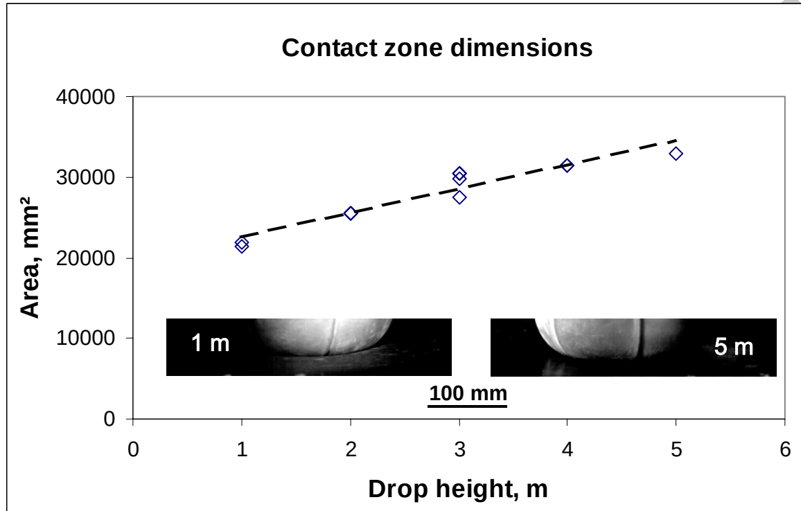
Figure 12. Influence of drop height on contact zone area. Images show ball form and correspond to maximum ball compaction for two drop heights onto pinned foam core sandwich.
