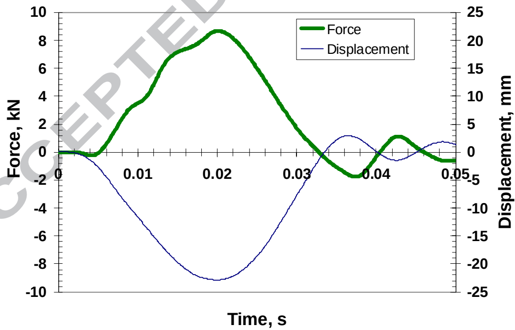
b) Pinned foam
