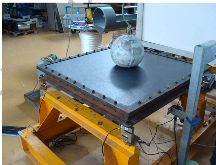
Figure 4. Test set-up. Upper: Support frame and 18.8 kg ball on one metre square panel
