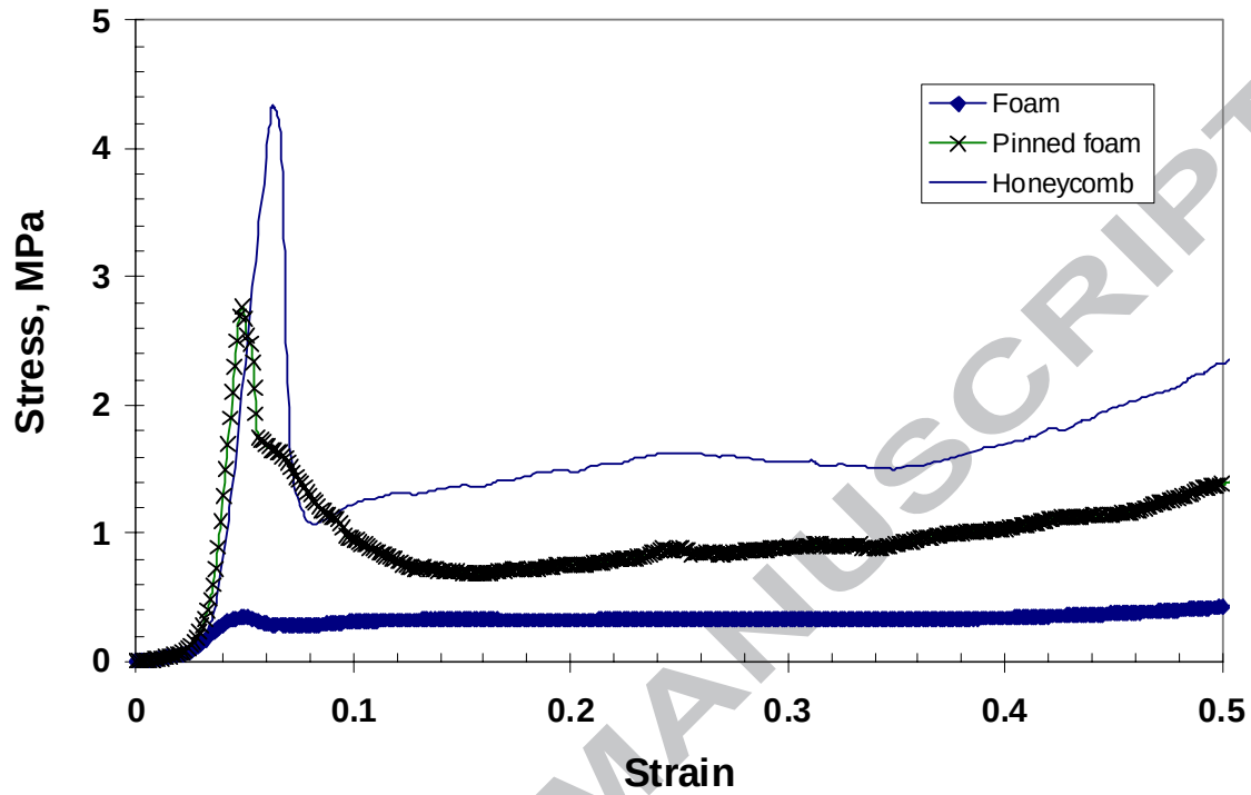
Figure 5. Representative stress-strain curves, quasi-static compression tests.
