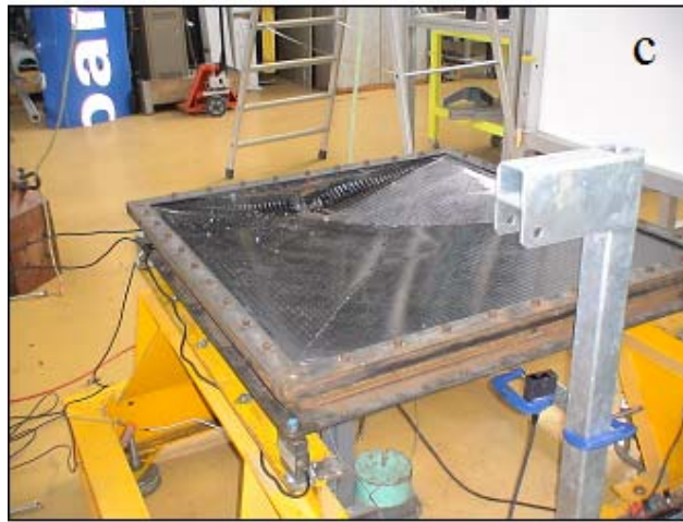
Figure 9. Damage observed after impact
