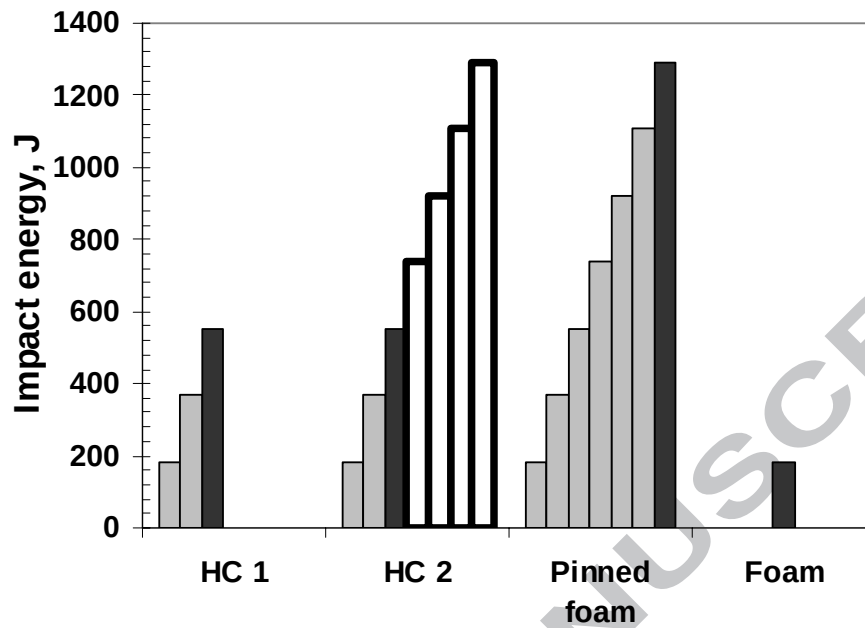
Figure 8. Impact tests performed; HC: Honeycomb. Grey indicates undamaged, black indicates first panel damage noted, white columns indicate panel tests continued after first damage.
