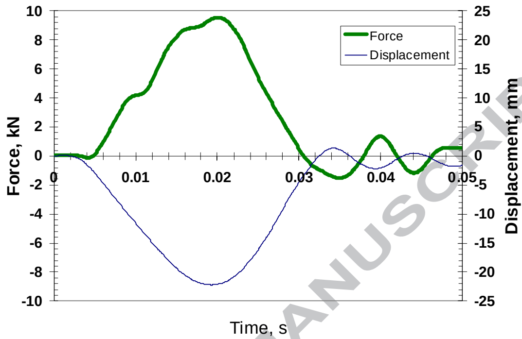
a) Honeycomb 64 kg/m 3
