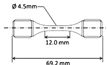
3 Round bar low cycle fatigue test specimen schematic
