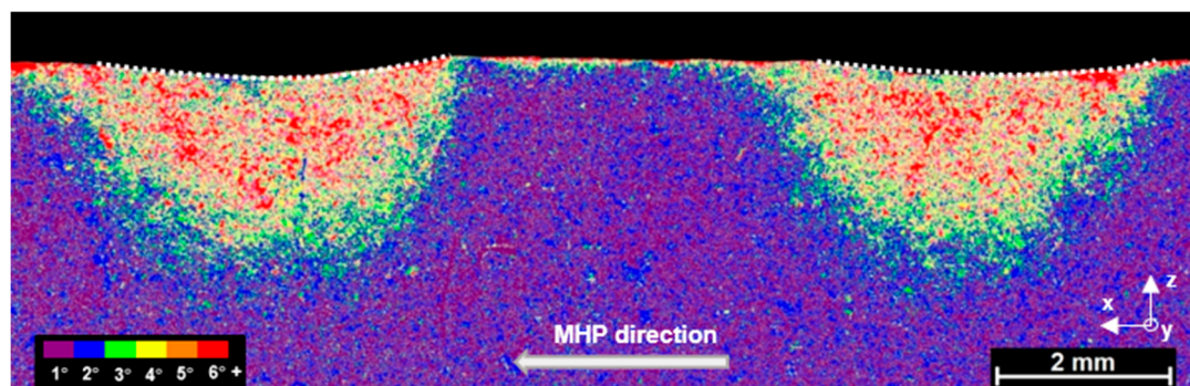
Figure 17. Overlaid \beta -reconstructed EBSD maps accepting increasing deviation from the ideal BOR (1–6°) to infer the plastic strain distribution of two impacts for peening step size of 8 mm and radius of 10 mm.
