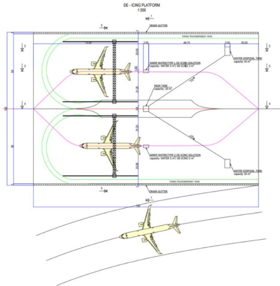
Figure 4 – Designated platform design for the airport. The AIHCB-compatible platform accommodates dual aircraft de-icing for Category C planes, with an alternate route for larger aircraft. Located 220m from runway 08R, it features a drain system leading to 30m 3 disposal tanks for efficient fluid management, minimizing maintenance. Safety buffers of 6m prevent collisions. Equipped with perimeter lighting and a backup generator, operations remain visible and uninterrupted, even at night. Pink lines guide aircraft to the system, while red and green lines manage queueing and emergency towing truck paths. In case of system failure, manual de-icing trucks can be refilled from the tanks.
