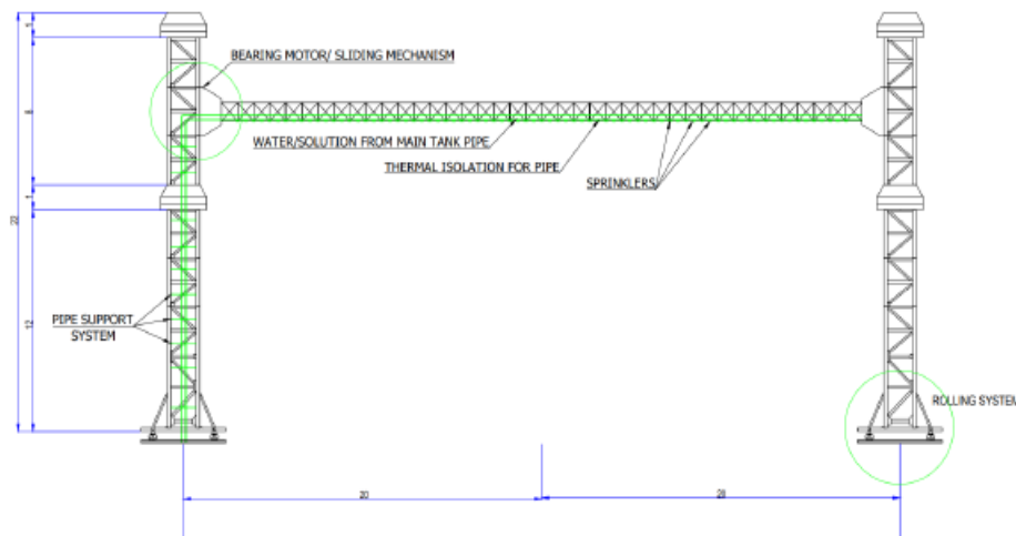
Figure 3 – Proposed Automated De-icing System Prototype Design. The design features a metal crossbar structure for airflow and cost efficiency. The platform moves on electrified rails to position over aircraft, adjusting in height via a motorized sliding rod mechanism up to 7.8m with 1m safety buffers. Equipped with advanced sensors, the system disperses de-icing fluid from a thermally insulated main tank through high-pressure nozzles for precise application.
