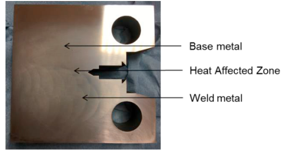
Fig. 2. C(T) specimen extracted from the welded slice
