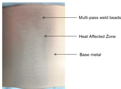
Fig. 1. Cross-weld extracted slice after polishing and etching of the surface
