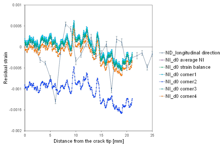
Fig. 6. Residual strains within the HAZ using neutron diffraction and neutron imaging techniques with different d_0
