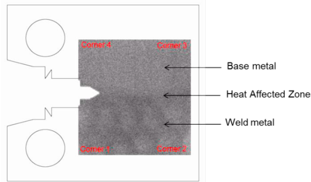
Fig. 5. Neutron radiography of the C(T) sample and the d_0 location with respect to the BM, HAZ and WM
