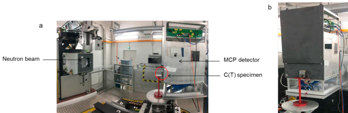
Fig. 4. (a) Neutron imaging experimental set up on IMAT; (b) C(T) specimen in front of the MCP detector
