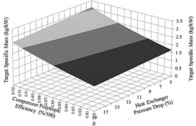
Target Specific Mass vs Compressor Polyropic Efficiency vs Heat Exchanger Pressure Drop for Double Stage RBCC (10 kW cold load, 20 K operation temperature, LCH 4 heat sink at 110 K)
