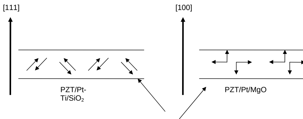
Relative orientation of domains in the PZT thin
