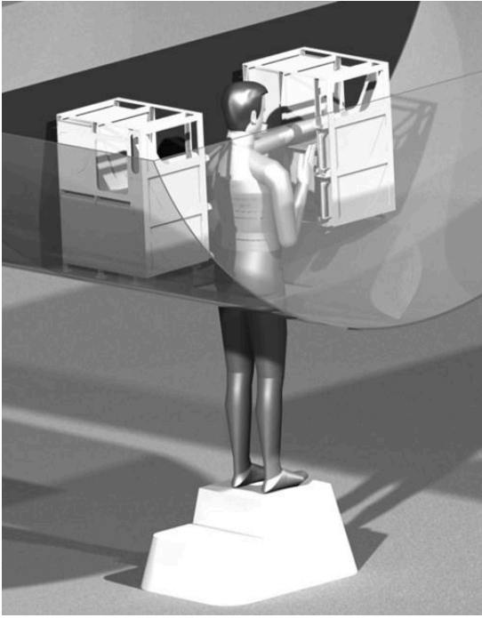
Figure 6: Redesigned A-8 Avionics Bay with 5 th Percentile Maintainer.
