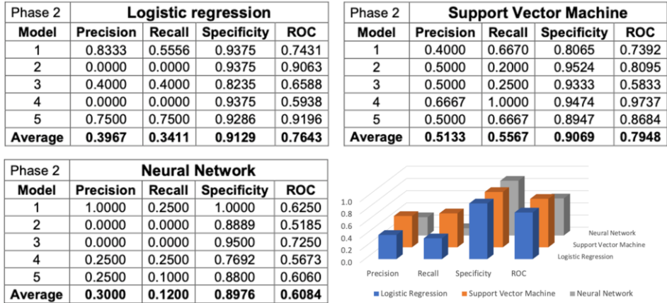
Figure 1. Results comparing the three different ML algorithms.
