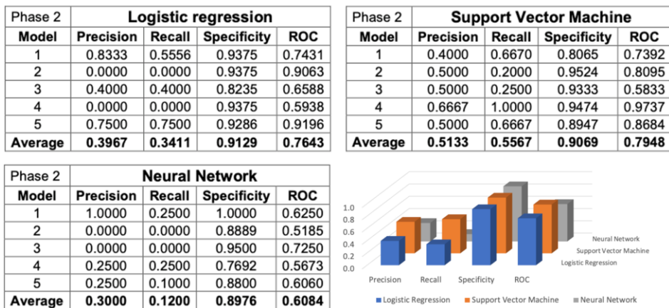
Figure 1. Results comparing the three different ML algorithms.
