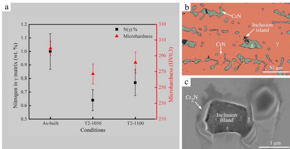
Fig. 11. (a) Changes of nitrogen concentrations in the γ matrix (N(γ)%) and microhardness of the as-built, T2-1050 and T2-1100 conditions (N(γ)%) was measured by EDS detector and at least three points were taken for every sample), (b) EBSD phase diagram for the T2-1050 sample showing the austenite (ochre), ferrite (cyan), CrN (yellow) and inclusions (black), (c) rod-like Cr 2 N precipitations around the inclusion island after condition T2-1100. (STEDVP was chosen for the calculation of error bars).
