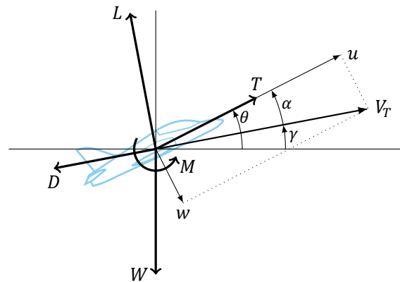
Figure 3. Configuration for 3-DOF aircraft longitudinal dynamics.
