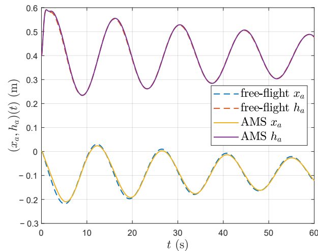
Figure 10. Phugoid mode height and lateral surge position response of the free-flying Hawk model (resolved into the wind tunnel axes) and the aircraft-manipulator system (AMS) model.
