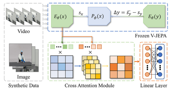
Fig. 2. Training paradigm of the proposed method. The frozen V-JEPA model is used to extract features from the synthetic dataset, and the final classification is performed through a linear projection layer.
