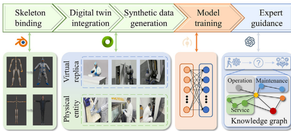
Fig. 1. An overview of the proposed Sim2Know framework. Three key contributions include synthetic data generation through digital twins (DT), action recognition training and in-depth knowledge provision through a knowledge graph (KG).
