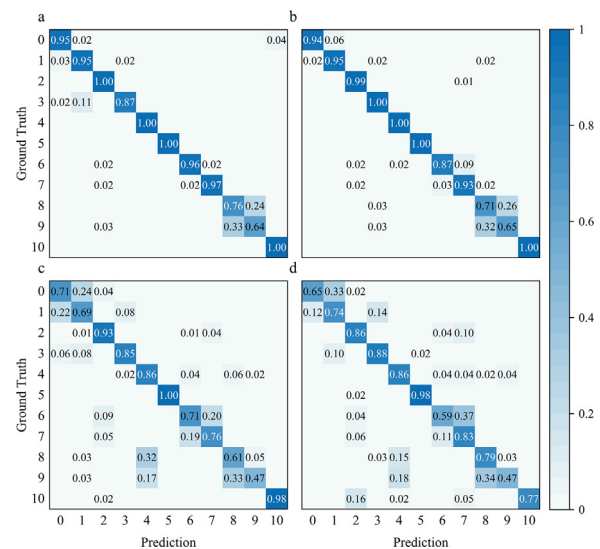
Fig. 3. Confusion matrices showing action recognition performance across different training configurations (index from 0~10 refers to 11 actions). (a) video dataset at 384^2 , (b) video dataset at 224^2 , (c) image dataset at 384^2 , and (d) image dataset at 224^2 .
