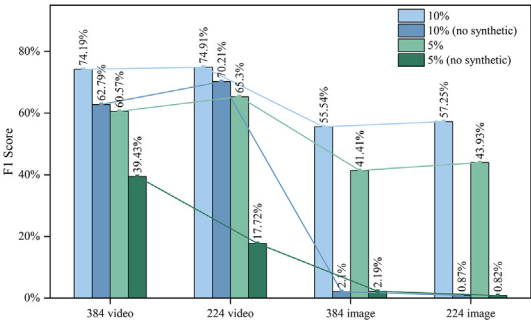
Fig. 4. Performance comparison (F1 scores) across training configurations with varying real data ratios (5 %–10 %) with and without the integration of synthetic data.
