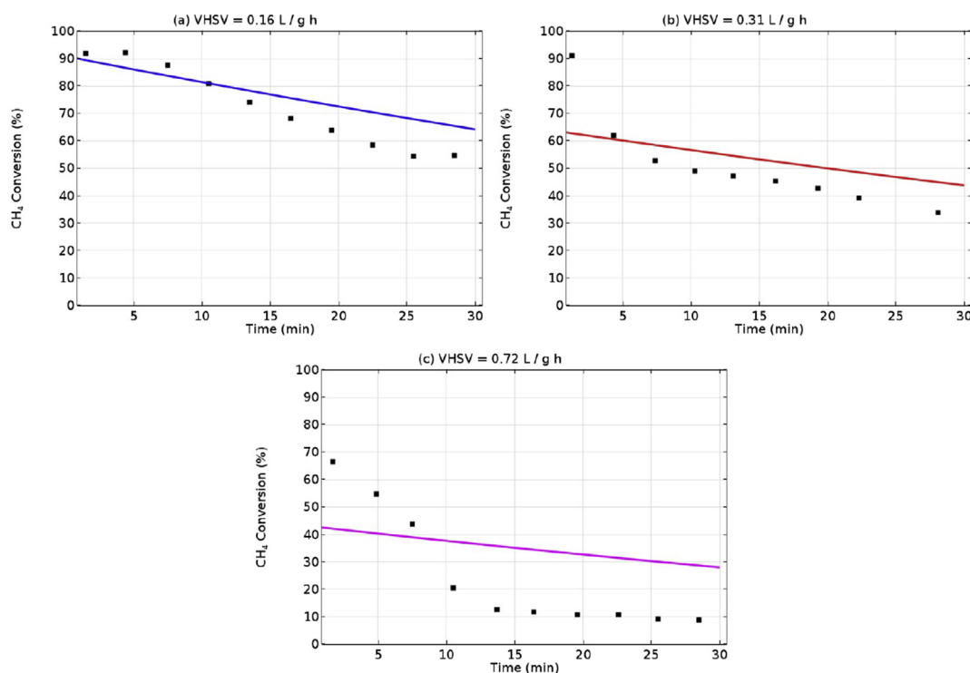
Fig. 6 – \text{CH}_4 conversion as a function of time for three different VHSV values, (A) 0.16 L/(g h), (B) 0.31 L/(g h) and (C) 0.72 L/(g h). Square markers represent the experimental data and continuous lines represent the simulation predictions.
