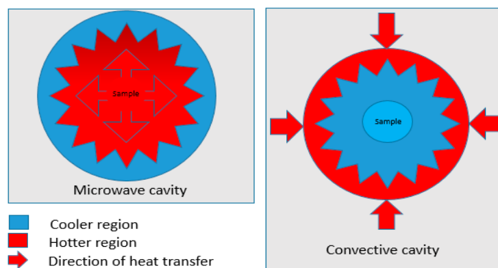
Figure 3. Examples of conventional and microwave heating effects.
