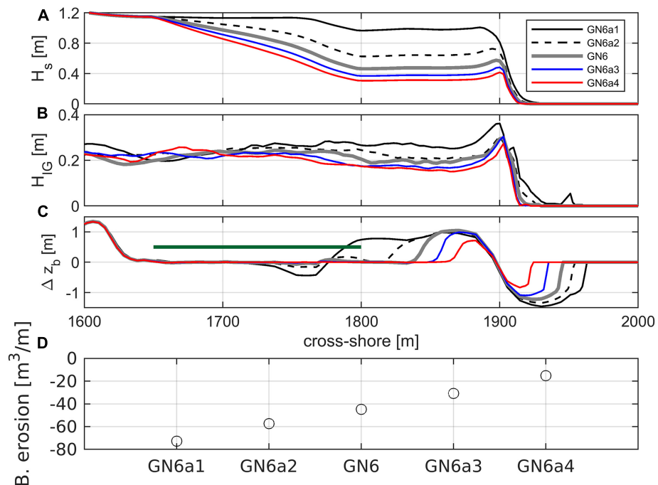
FIGURE 11 | Sensitivity to seagrass height ah , showing: (A) wave height distribution; (B) infragravity wave distribution; (C) seabed change after 100 days simulation; and (D) beach erosion.
