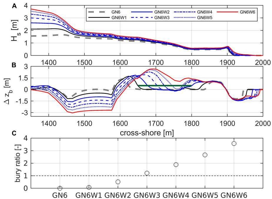
FIGURE 10 | Sensitivity of seagrass to offshore wave conditions, showing: (A) wave height distribution; (B) seabed change after 100 days simulation; and (C) meadow averaged bury ratio.
