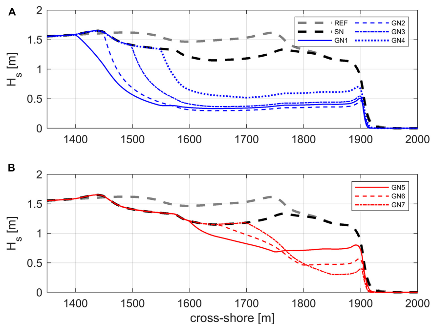
FIGURE 3 | Cross-shore wave height distribution under mild wave (i.e., H_m = 1.5 m, T = 8 s) for: (A) case REF, SN, GN1-4; and (B) case GN5-7.
