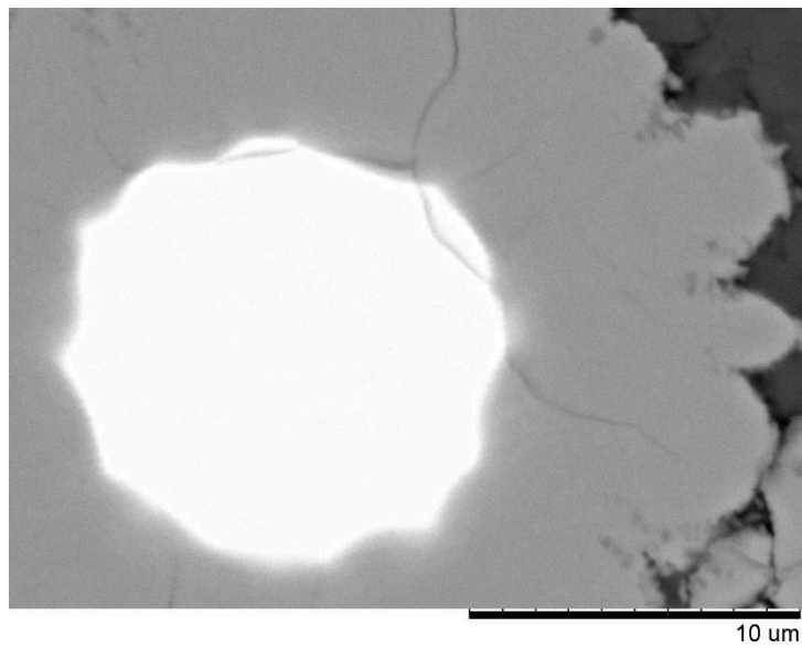
Figure 12. Reaction layer forming at the interface in composites obtained from the Al–20 vol.% \text{Fe}_{66}\text{Cr}_{10}\text{Nb}_5\text{B}_{19} powder mixture: (a) SPS at 570 °C and (b) SPS at 500 °C followed by annealing at 570 °C.
