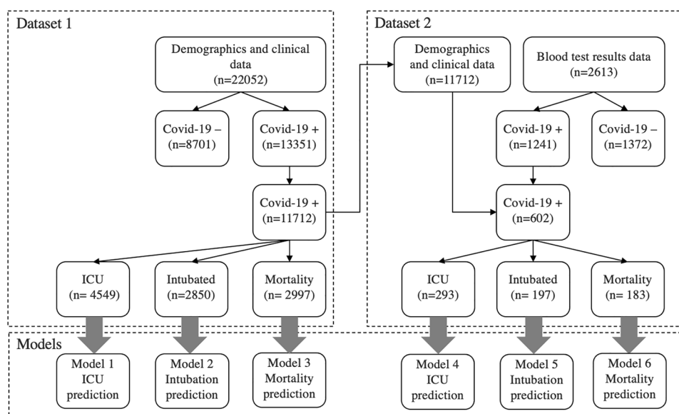
Fig. 1 Datasets used to develop the prediction models
