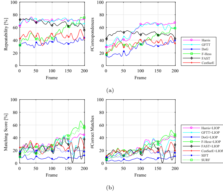
Figure 12: Performance for rendezvous sequence: successive transformations, visible band, hot case. (a) Repeatability and number of correspondences. (b) Matching score and number of correct matches. The raw data is presented smoothed with markers added for readability. The dashed lines show the results for DoG and Fast-Hessian with their original descriptor.
