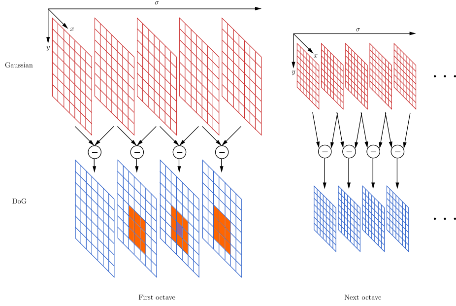
Figure 2: The difference of Gaussian pyramid structure (adapted from [21]). Adjacent Gaussian images are subtracted to produce the DoG images, each octave is characterised by down-sampling the previous one by a factor of 2. Features are selected in the DoG images by comparing a candidate point (purple) to its neighbours (orange) in scale and space.
