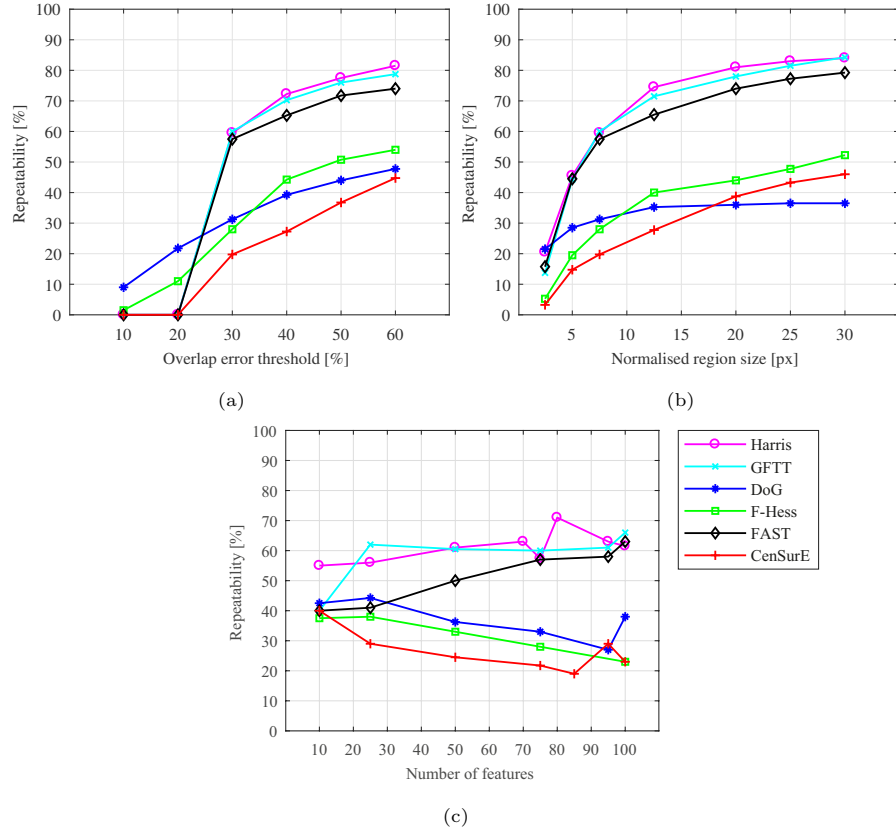
Figure 11: Repeatability scores as a function of different benchmark parameters. (a) Repeatability vs overlap error threshold. (b) Repeatability vs normalised region size. (c) Repeatability vs region density.
