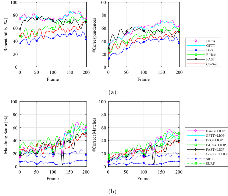
Figure 16: Performance for rendezvous sequence: successive transformations, thermal infrared band, hot case. (a) Repeatability and number of correspondences. (b) Matching score and number of correct matches. The raw data is presented smoothed with markers added for readability. The dashed lines show the results for DoG and Fast-Hessian with their original descriptor.
