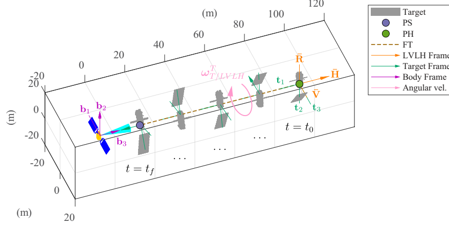
Figure 6: Scenario specifications for dataset generation, centred in the chaser's body frame \mathcal{F}_B . The relative configurations of the target frame \mathcal{F}_T and of the LVLH frame are shown.
