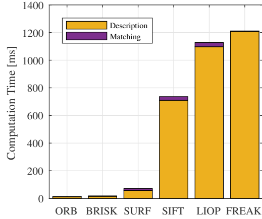
Figure 25: Comparison of average feature description and matching times per frame.
