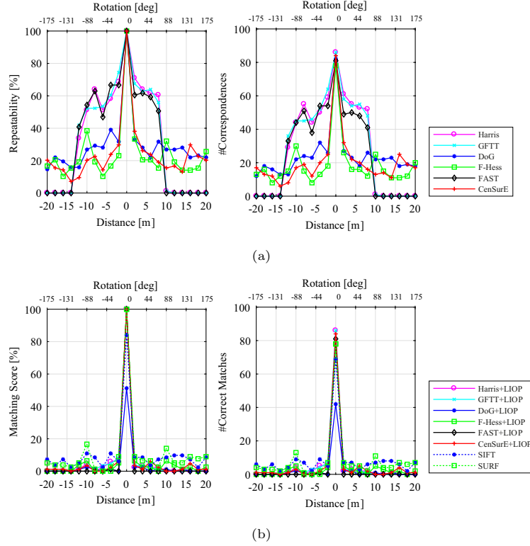
Figure 15: Performance for rendezvous sequence: large transformations, visible band, cold case. (a) Repeatability and number of correspondences. (b) Matching score and number of correct matches. The dashed lines show the results for DoG and Fast-Hessian with their original descriptor.
