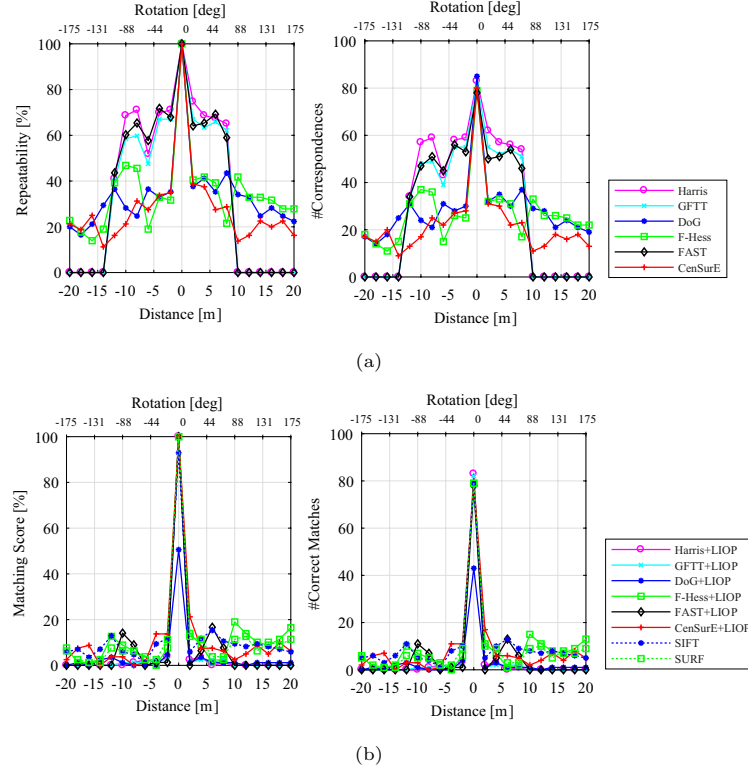
Figure 17: Performance for rendezvous sequence: large transformations, thermal infrared band, hot case. (a) Repeatability and number of correspondences. (b) matching score and number of correct matches. The dashed lines show the results for DoG and Fast-Hessian with their original descriptor
