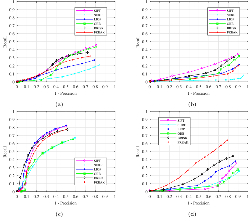
Figure 23: Descriptor ROC curves for the thermal infrared band, cold case. (a, b) DoG features with small and large transformations. (c, d) Fast-Hessian features with small and large transformations.
