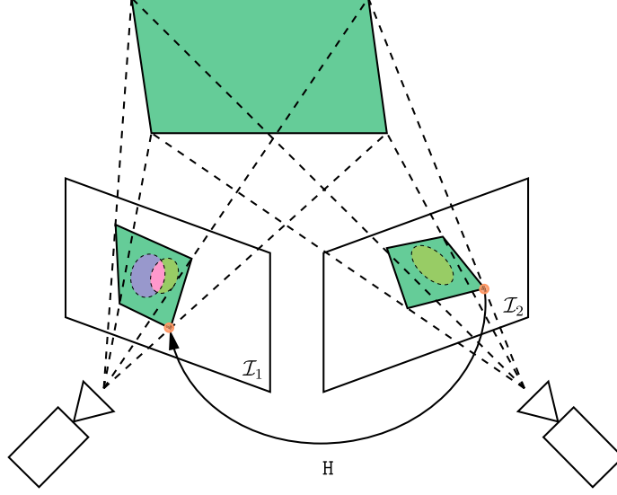
Figure 4: The homography ground truth \mathbf{H} maps the light green feature from frame \mathcal{I}_2 to frame \mathcal{I}_1 . The overlap area with the original purple feature from \mathcal{I}_1 is shown in pink. If the amount of overlap is above a certain defined threshold, then the two features correspond.
