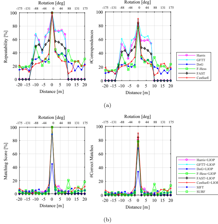
Figure 19: Performance for rendezvous sequence: large transformations, thermal infrared band, cold case. (a) Repeatability and number of correspondences. (b) Matching score and number of correct matches. The dashed lines show the results for DoG and Fast-Hessian with their original descriptor.
