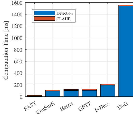
Figure 24: Comparison of average feature detection times per frame.
