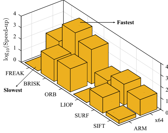
Figure 26: Comparison of descriptor speed-up factors in different processors.
