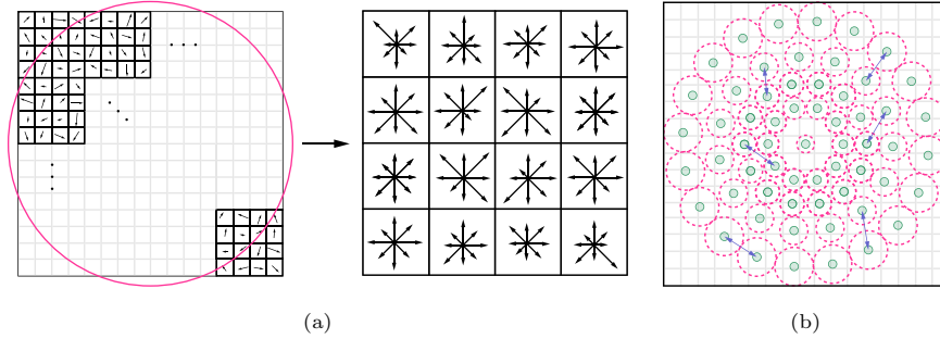
Figure 3: Distribution-based and binary description. (a, left) SIFT: the gradient magnitude and orientation at each subregion are weighted by a Gaussian window (pink) and (a, right) accumulated into a histogram (adapted from [21]). (b) BRISK: sampling locations (green) and Gaussian kernels to smooth intensity values (pink) for n = 60 points and some pairwise comparisons (purple) between them (adapted from [27]).
