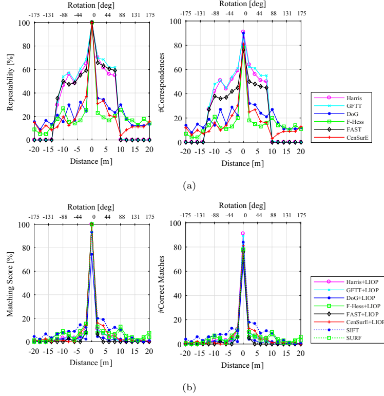
Figure 13: Performance for rendezvous sequence: large transformations, visible band, hot case. (a) Repeatability and number of correspondences. (b) Matching score and number of correct matches. The dashed lines show the results for DoG and Fast-Hessian with their original descriptor.
