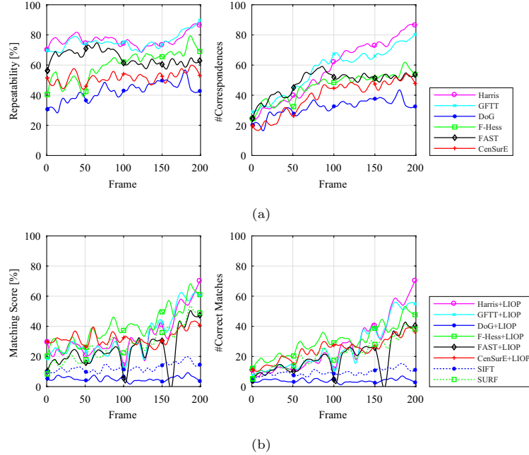
Figure 18: Performance for rendezvous sequence: successive transformations, thermal infrared band, cold case. (a) Repeatability and number of correspondences. (b) Matching score and number of correct matches. The raw data is presented smoothed with markers added for readability. The dashed lines show the results for DoG and Fast-Hessian with their original descriptor.
