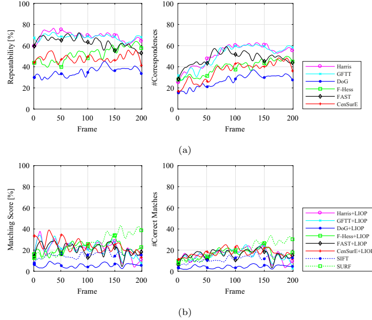
Figure 14: Performance for rendezvous sequence: successive transformations, visible band, cold case. (a) Repeatability and number of correspondences. (b) Matching score and number of correct matches. The raw data is presented smoothed with markers added for readability. The dashed lines show the results for DoG and Fast-Hessian with their original descriptor.
