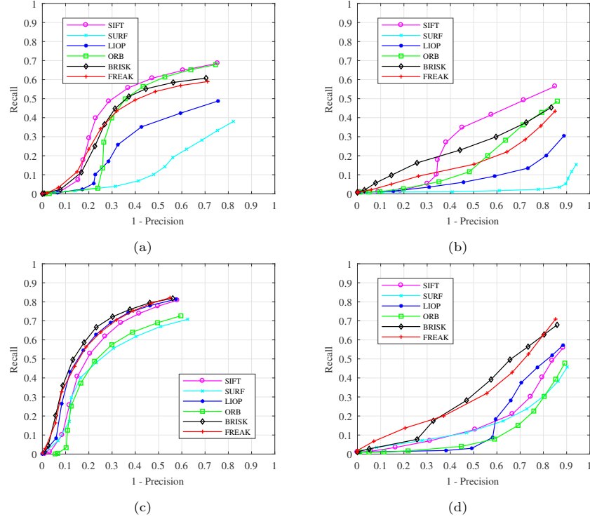
Figure 20: Descriptor ROC curves for the visible band, hot case. (a, b) DoG features with small and large transformations. (c, d) Fast-Hessian features with small and large transformations.
