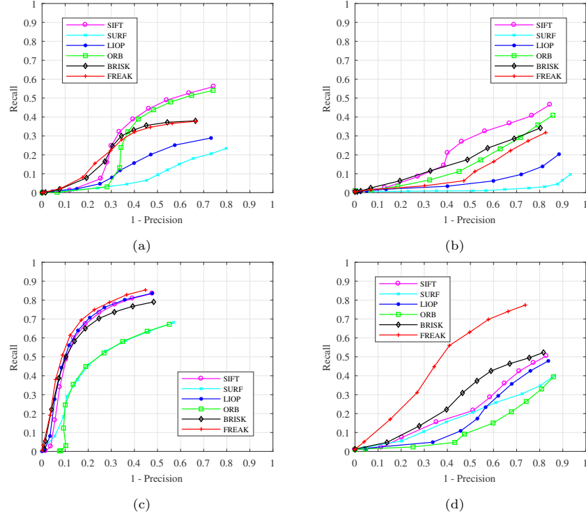
Figure 22: Descriptor ROC curves for the thermal infrared band, hot case. (a, b) DoG features with small and large transformations. (c, d) Fast-Hessian features with small and large transformations
