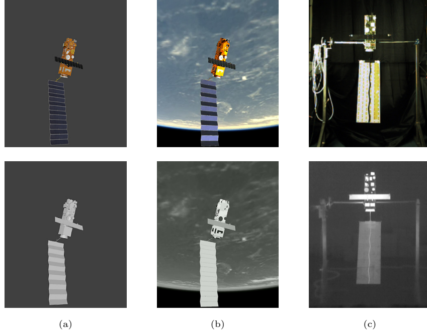
Figure 7: Multispectral modelling of Envisat. (top) Visible. (bottom) LWIR. (a) Original CAD mesh. (b) Modified mesh and materials running on the Astos engine. (c) Laboratory mock-up.
