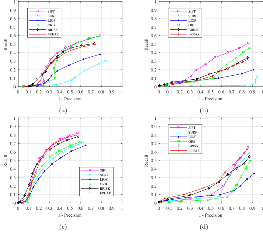
Figure 21: Descriptor ROC curves for the visible band, cold case. (a, b) DoG features with small and large transformations. (c, d) Fast-Hessian features with small and large transformations.
