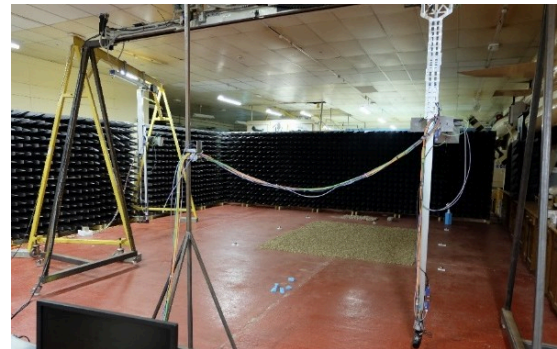
Figure 1. The GBSAR laboratory in a bistatic configuration, measuring a gravel scene.
