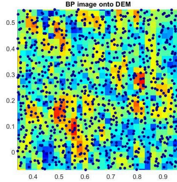
Figure 5 (b). Zoomed in view of a simulated SAR image with scatterer positions overlaid with dark blue dots.
