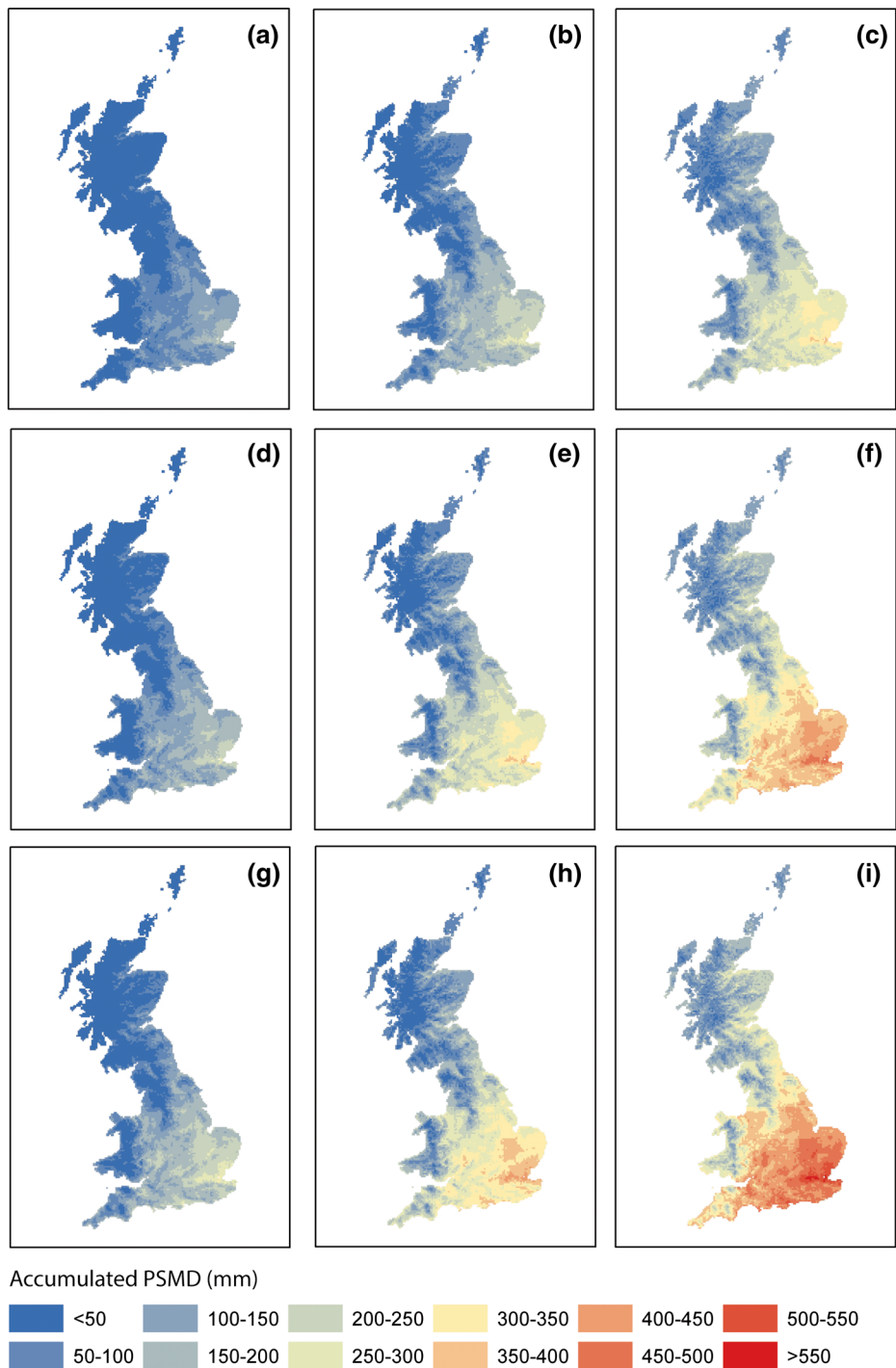
Fig. 4 UKCP09-derived projections of accumulated annual PSMD for GB Baseline (1961–1990) a 10th, b 50th and c 90th percentiles; 2030 (2020–2049) d 10th, e 50th and f 90th percentiles; 2050 (2040–2069) g 10th, h 50th and i 90th percentiles
