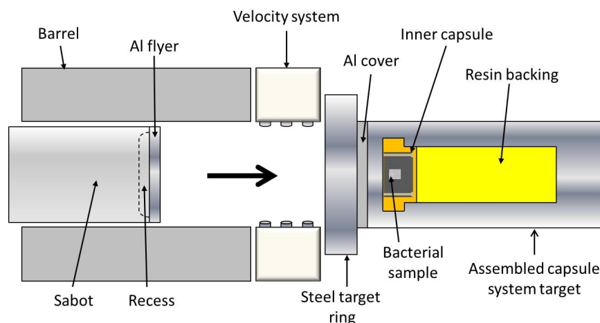
Figure 1. A basic diagram showing the target setup for shockwave experiments [9].
