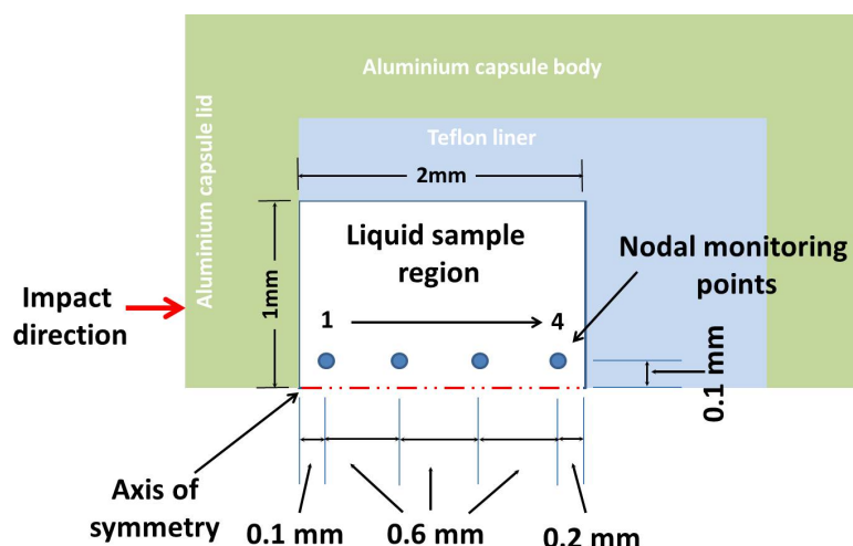
Figure 1. A basic diagram showing the target setup for shockwave experiments [9].
