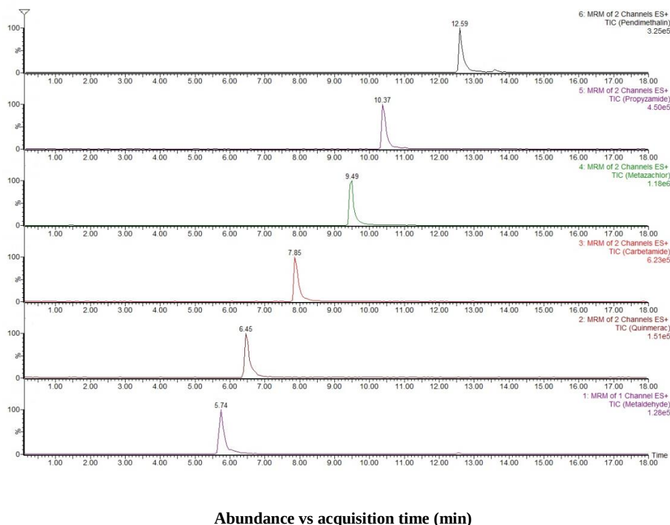
Figure 2. Example chromatograms of six pesticides at 10 µg L -1 in ultra-pure water by direct aqueous injection.
