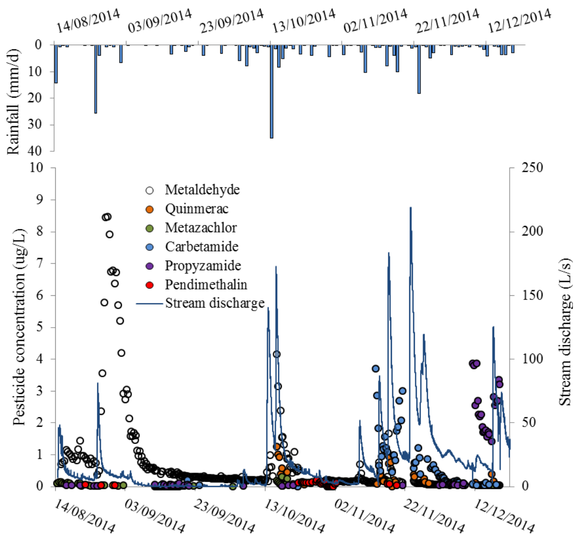
Figure 3. Rainfall (top panel), stream discharge (right axis) and pesticide concentrations (left axis) in the Hope Farm stream from August to December 2014.
