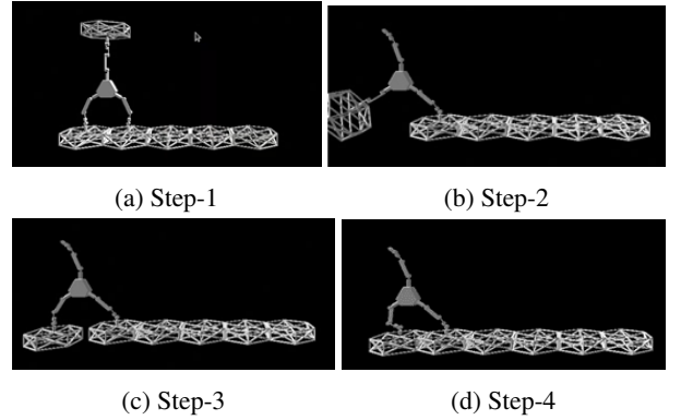
Figure 8: i^{\text{th}} SRS Assembly Steps
