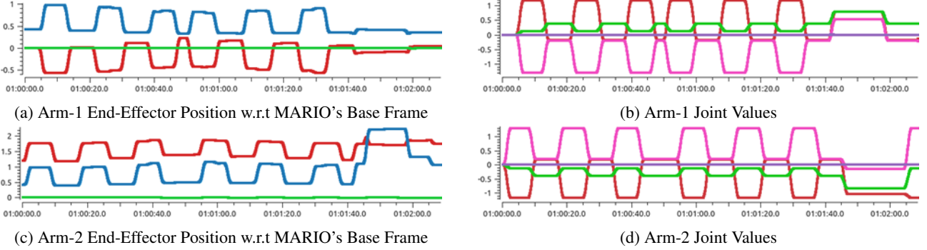
Figure 10: Position and Joint Values of Arm-1 and Arm-2 (Distance/Joint angles as a function of Simulation Time)
