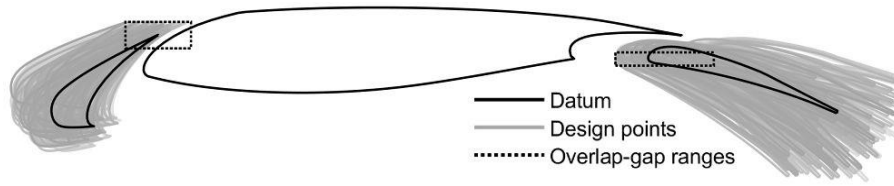
Figure 8 – MBO design space visualization.
