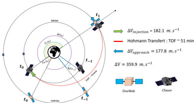
Figure 7 Co-planar rendezvous
