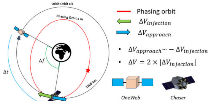
Figure 8 Co-orbital rendezvous
