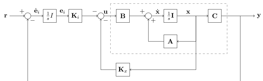
Figure 29. Draganflyer X-Pro quadrotor LQR control schematic with integral action.
