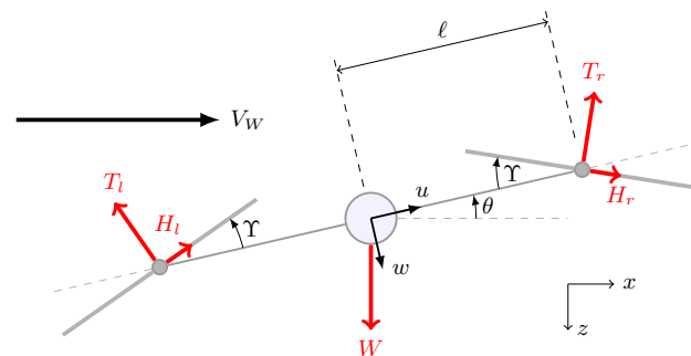
Figure 7. Schematic of the PVTOL vehicle including rotor tilt, \Upsilon .
