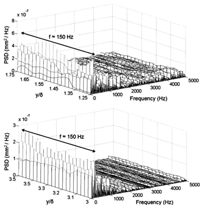
FIG. 5. Power spectral density plotted against frequency along locations (a) y/\delta=1.25 to y/\delta=1.75 and (b) y/\delta=3.0 to y/\delta=3.5 from Fig. 2.
