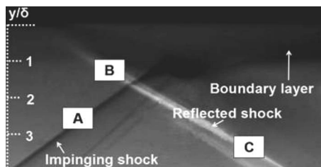
FIG. 2. Typical schlieren image of shock wave/turbulent boundary-layer interaction with separation indicating three different regions: A (incident shock), B (reflected shock upstream of impingement location), and C (reflected shock downstream of impingement location). Flow from left to right.
