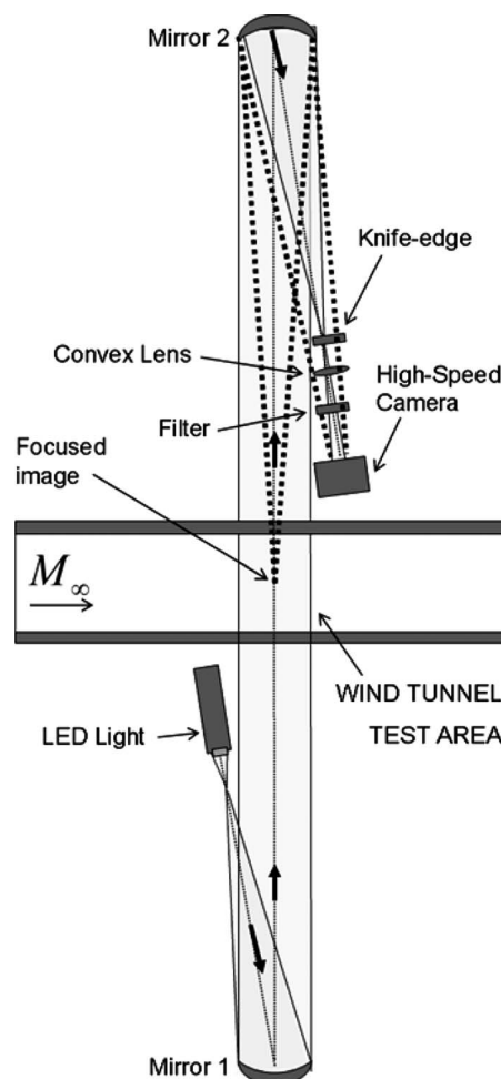
FIG. 1. Schematic diagram of high-speed schlieren optical arrangement.
