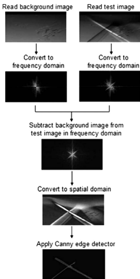
FIG. 3. Image processing routine including background image subtraction in the frequency domain to equally distinguish both dark and light shocks.
