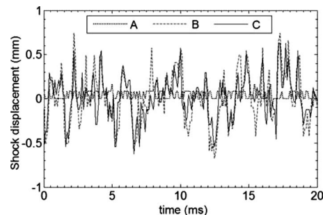
FIG. 4. Shock displacement (mm) as a function of time (ms), corresponding to locations A, B, and C from Fig. 2.
