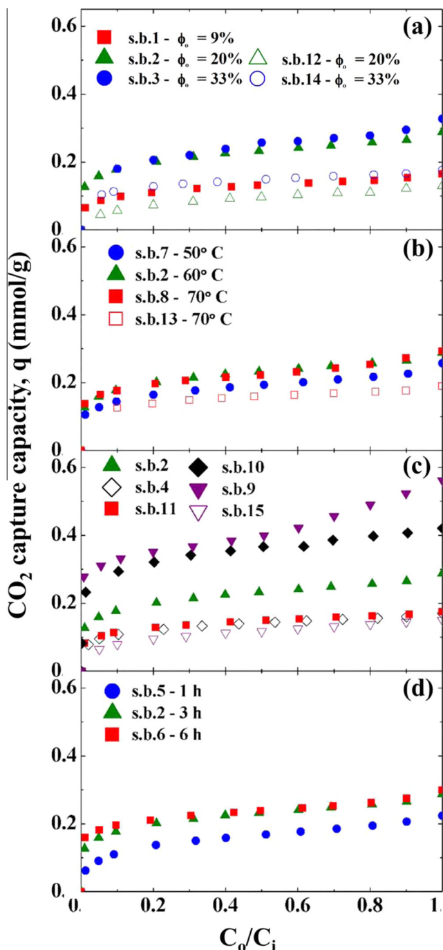
Fig. 8. The \text{CO}_2 adsorption capacity of the samples listed in Table 1 calculated from the breakthrough curves using Eq. (2). The variable parameter: (a) disperse phase volume fraction; (b) polymerization temperature; (c) template concentration, solvent content, and monomer concentration in the organic phase; (d) polymerization time. The adsorption temperature was 40^\circ\text{C} and the gas flow rate was 130\text{ mL/min} for all runs. For (a–c) the filled symbols represent MIP samples, and the empty symbols represent the corresponding NIP samples.
