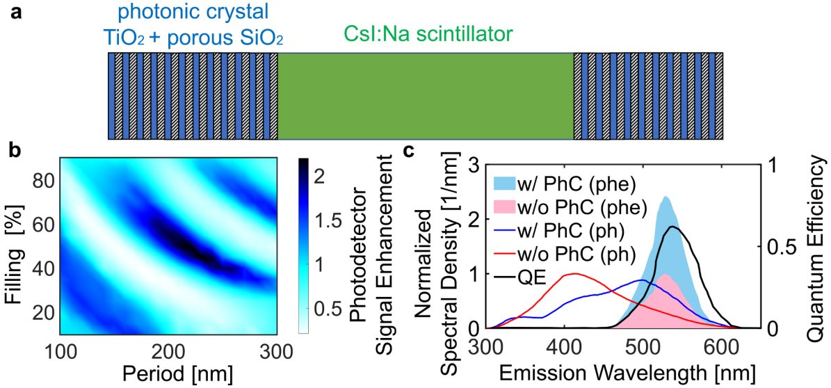
Figure 4. External photonic crystal (PhC) cavity-enhanced scintillator system using actual materials. (a) Schematic diagram of Csl:Na scintillator with a PhC cavity ( \text{TiO}_2 + porous \text{SiO}_2 ). The \text{TiO}_2/\text{SiO}_2 PhCs have been shown to be feasible in previous work. 48 Here, we replace \text{SiO}_2 film with \text{SiO}_2 porous material so as to achieve a low refractive index (1.06) 47 for the \text{SiO}_2 layer. \text{SiO}_2 porous material can be realized by random \text{SiO}_2 nano-rod arrangement. (b) Photodetector signal enhancement vs. period & filling factor of photonic crystal. (c) Spectral density of photons (ph) & photoelectrons (phe) with optimized configuration of PhC cavity ( \text{TiO}_2 + porous \text{SiO}_2 ). The emission spectrum is shifted to longer wavelength to match the quantum efficiency (QE) spectrum of the photo-detector. The enhancement of the overall photodetector signal is 121%.
