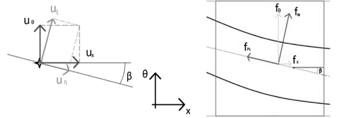
(a) Vectors along camberline direction (b) Body force composition
