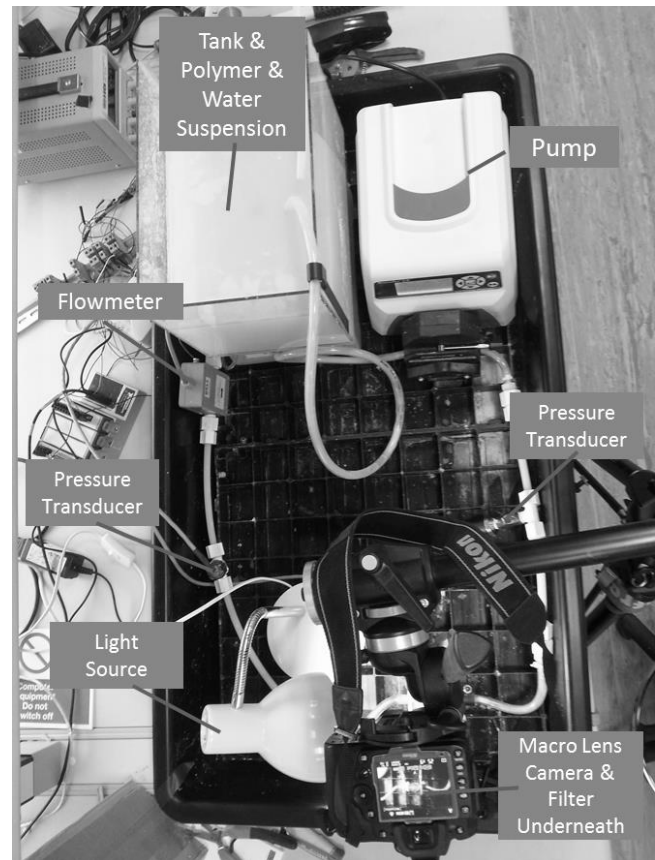
Figure 4. Filter clogging test rig &amp; components
