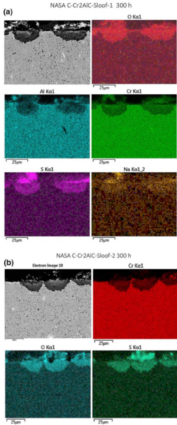
Fig 13. Elemental SEM/EDS rasters for hot corrosion tested (C) 100% dense \text{Cr}_2\text{AlC} sample after 300 h at 700°C showing Al-oxide outer nodule, Cr-oxide inner pit, both intermingled with residual Na-S-O.
