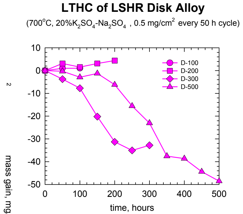
Fig 4. Progressive 700°C LTHC weight change of four (D) LSHR disk superalloy samples. Eventual weight loss indicates repeated spallation of thick corrosion layers. 0.5 mg/cm 2 20 K 2 SO 4 -80Na 2 SO 4 deposited every 50 h. (Dashed line indicates approximate salt loading weight).
