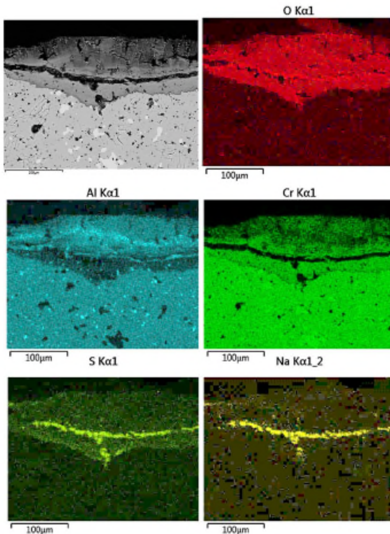
Fig 11. Elemental SEM/EDS rasters for hot corrosion tested (A) Kanthal Cr 2 AlC-3 sample after 500 h at 700°C showing Al-oxide outer, Cr-oxide inner, and residual Na-S-O mid layers.
