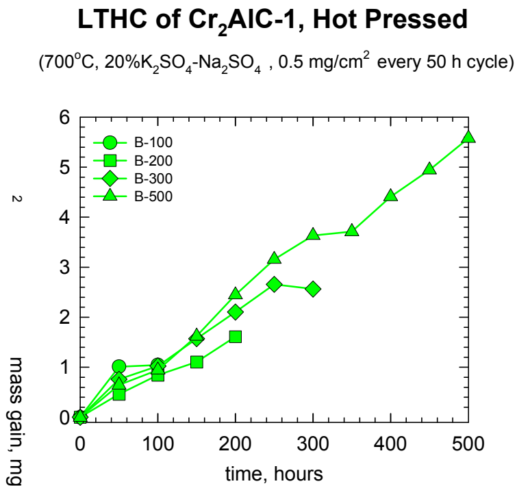
Fig 2. Progressive 700°C LTHC weight change of four hot pressed (B) Kanthal Cr 2 AlC-1 samples. Little indication of excessive growth or spallation. 0.5 mg/cm 2 20K 2 SO 4 -80Na 2 SO 4 deposited every 50 h. (Dashed line indicates approximate salt loading weight).
