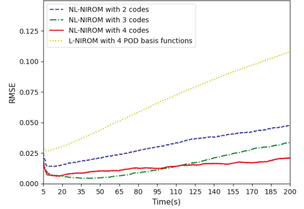
(b) RMSE
