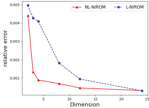
Figure 11: Case 1: Flow past a cylinder. The relative error of velocity between the full model and two NIROMs against their dimensional size in reduced space.
