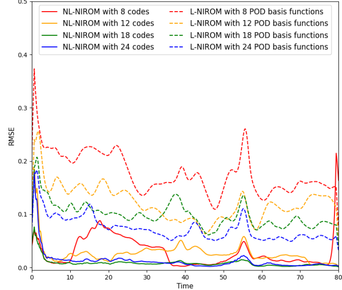
(b) RMSE
